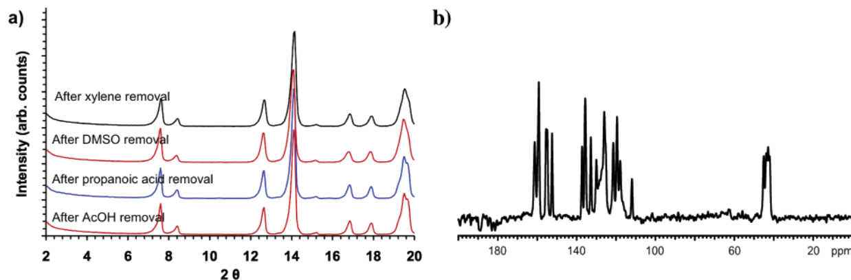
Figure 14. (a) Comparison of the PXR D patterns for apohost 1 formed after removal of a variety of guest molecules from host 1 ·guest. (b) Ramped ^{13}\text{C}(^1\text{H}) CP-MAS NMR spectra for the crystalline apohost 1 .
