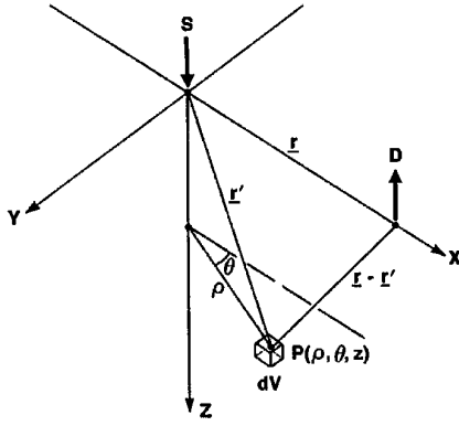
Fig. 1. Geometry for calculation of the relative visit probability in absorption spectroscopy. The light source (S) is a collimated pencil beam incident on the tissue at the origin, and a detector (D) is located at \mathbf{r} on the tissue surface (the x - y plane). For the simple diffusion model it is assumed that all photons are isotropically scattered at a depth z_0 on the z axis. As explained in the text, the fluence rate is assumed to be zero on a plane parallel to and above the tissue surface at z = z_p . The goal of the calculation is to determine the change in signal at the detector resulting from a perturbation in the absorption coefficient in dV near P(\rho, \theta, z) .
