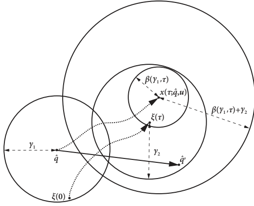
Figure 1: Proposition 1 provides concrete means to over-approximate \rightarrow_{\tilde{\tau}_c} by adding (\hat{q}, \mathbf{u}, \hat{q}') to \rightarrow_{\tilde{\tau}_c} whenever |\hat{q}' - x(\tau; \mathbf{u}, \hat{q})| \leq \beta(\gamma_1, \tau) + \gamma_2 . In view of condition (4), the ball B_{\beta(\gamma_1, \tau)}(x(\tau; \hat{q}, \mathbf{u})) includes \xi(\tau) for all \xi : [0, \tau] \rightarrow \mathbb{R}^n such that |\xi(0) - \hat{q}| \leq \gamma_1 and \dot{\xi}(s) = f(\xi(s), \mathbf{u}(s)) for all s \in [0, \tau] . Hence, the ball B_{\beta(\gamma_1, \tau) + \gamma_2}(x(\tau; \hat{q}, \mathbf{u})) contains all \hat{q}' \in \hat{Q} that is \gamma_2 -close to \xi(\tau) for some \xi defined above; that is, all \hat{q}' \in \hat{Q} such that (\hat{q}, \mathbf{u}, \hat{q}') \in \rightarrow_{\tilde{\tau}_c} as required by Definition 1.
