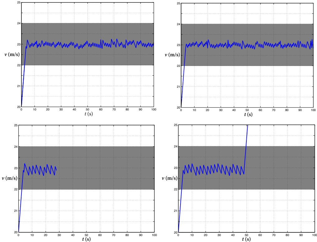
Figure 4: Simulation results for the cruise control example (11), where the system is subject to measurement errors bounded by \varepsilon = 0.1 and a delay in sensing, computation, and actuation bounded by h = 0.01 . We use an (\eta, \gamma_1, \gamma_2, \delta) -abstraction (given by Definition 1) of (11) to synthesize a hybrid control strategy. The upper two figures show simulated trajectories generated by a controller synthesized using an (\eta, \gamma_1, \gamma_2, \delta) -abstraction with \eta = 0.05 , \gamma_1 = 0.1674 , \gamma_2 = 0.15 , and \delta = 0.5947 , where \gamma_i ( i = 1, 2 ) are used to account for measurement errors and delays as shown in Theorem 3. The grey band indicates the desired speed range [22, 24]. The delays and measurements are randomly generated, which clearly led to somewhat random trajectories as opposed to periodic ones. The lower two figures show what could happen if measurement errors and delays are not accounted for within the abstractions, where we have chosen \gamma_1 = \gamma_2 = \eta = 0.05 , while \delta is kept the same. The lower left figure shows a termination of simulation when the measured system state, due to uncertainties in measurements, is mapped to an unexpected discrete state in the controlling automaton. One may keep executing the previous control input if the measurement is unexpected, but this may lead to violation of system specification as shown in the lower right figure.
