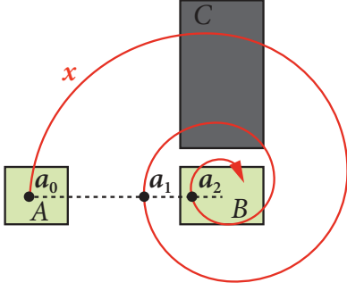
Figure 2: A simple illustration of inter-sample behaviors that violate a given specification, while a sampled sequence satisfies the same specification.
