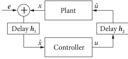
Figure 3: Illustration of a controller that takes delayed (by h_1 ) and imperfect measurement (subject to measurement errors bounded by \varepsilon ) from a plant and sends a control input that is received by the plant after another delay h_2 (measured from when the controller receives the measurement and to when the control input has been actuated by the plant). The total round-trip delay h_1 + h_2 is not assumed to be constant, but assumed to be bounded by some constant h . While the plant is waiting for the next control input, it keeps on executing the previous one.
