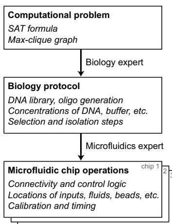
Figure 1: Abstraction layers for DNA computing.
