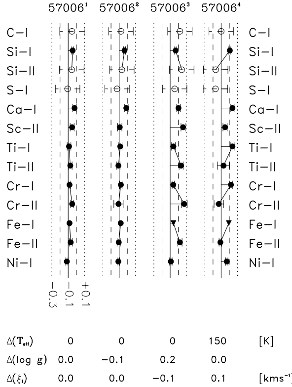
Fig. 6. Abundances for selected elements for four different models for HD 57006. See caption of Fig. 5 for details.
