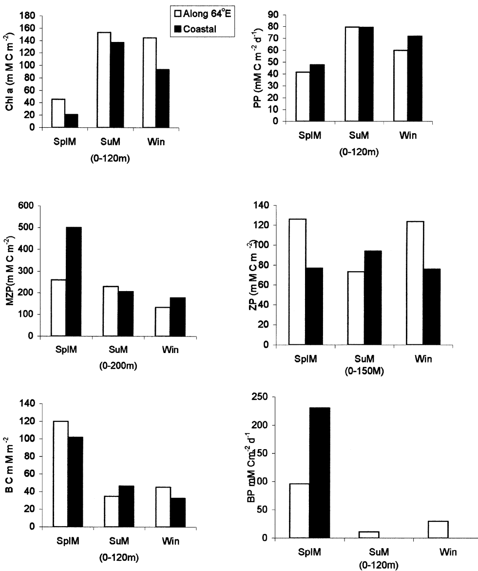
Figure 7. Living component carbon biomass in the sampling locations along 64°E and a transect along the west coast of India within 200m depth contour. Carbon biomass is in mM C m -2 . PP denotes primary production; MZP, microzooplankton; ZP, mesozooplankton; BC, bacterial carbon standing stock; BP, bacterial production; SpIM, spring intermonsoon; SuM, summer monsoon and, Win denotes winter.
