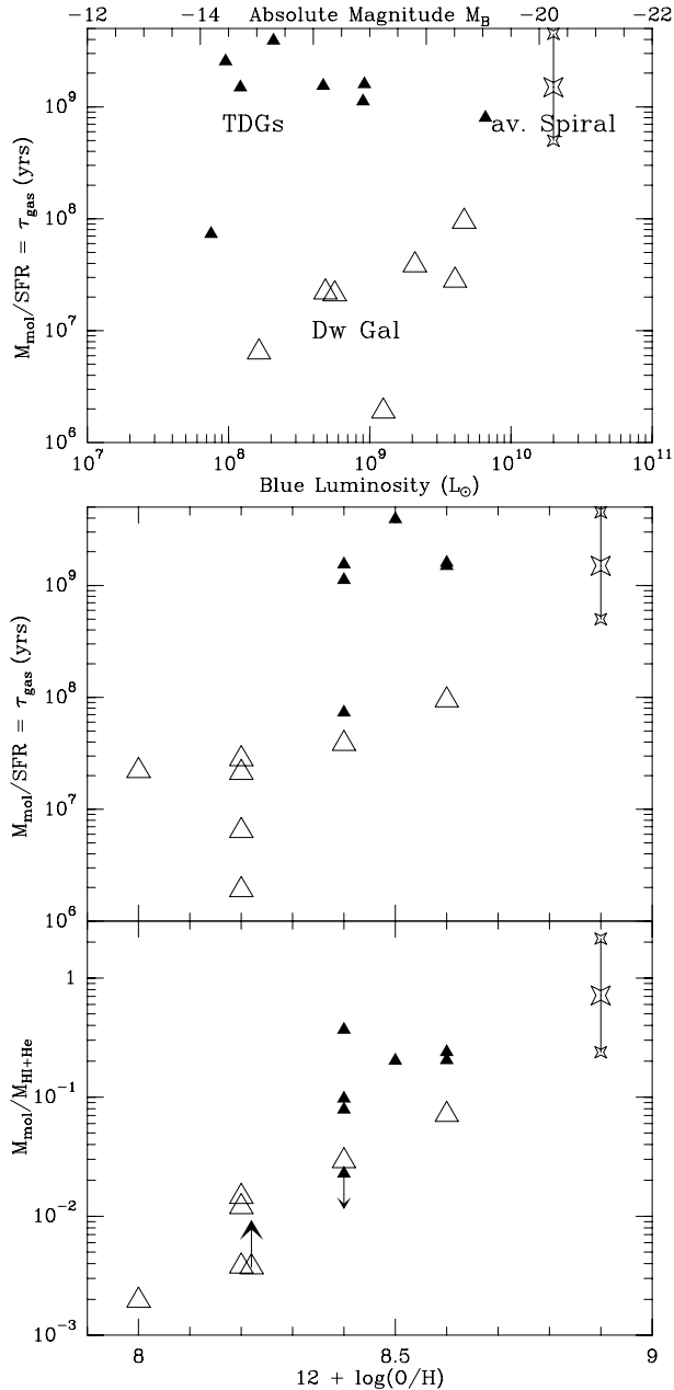
Fig. 8. (Top): comparison of gas consumption time, M_{\text{mol}}/\text{SFR} , which is the inverse of the frequently used Star Formation Efficiency (SFE), as a function of blue luminosity for the different categories of galaxies. Small filled triangles represent the TDGs (data from Tables 2 and 5), open triangles the regular dwarf galaxies (data from Table 4), and the star an average spiral as taken from Kennicutt (1998), similar in position on the diagram to the Milky Way. For Arp 245N values are for the CO-detected area, not just the center. The smaller stars give the range for “average” spirals. (Middle): as above but as a function of oxygen abundance. (Bottom): molecular to atomic gas mass ratios as a function of oxygen abundance. NGC 4214 has been moved slightly to the right to make it visible and the up arrow is because the HI mass is for a substantially greater area than covered by the CO observations. The same N(\text{H}_2)/I_{\text{CO}} value has been used for all galaxies, irrespective of metallicity or other influences, so M_{\text{mol}} is likely underestimated by a varying factor for the non-TDG dwarf galaxies.
