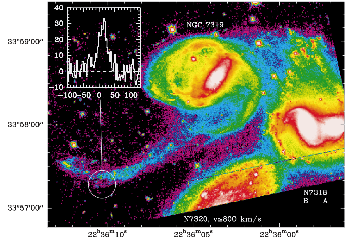
Fig. 6. Hubble Space Telescope V -band mosaic of Stephan’s Quintet. Spectrum is CO(1–0) emission and the circle marks the position observed in CO, which is the HI column density peak as observed by Shostak (1984). The zero velocity corresponds to cz = 6600 \text{ km s}^{-1} . NGC 7320 is a foreground galaxy.
