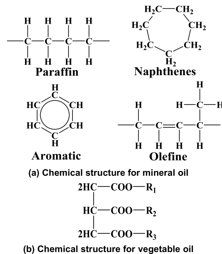
FIGURE 3. Chemical structure for mineral oil molecule and vegetable oil molecule.
