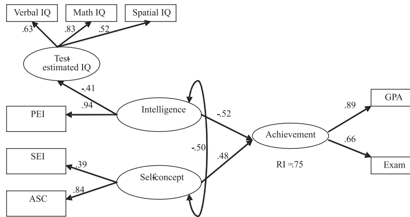
Figure 1. A diagram for the fitted SEM-model:
