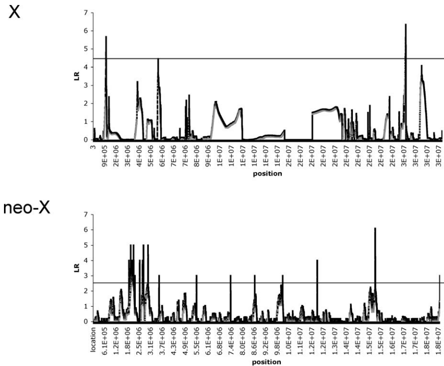
Figure 2. The Maximized Composite Likelihood Surface Calculated for Genes from the Ancestral X and the Neo-X Chromosome. The horizontal line indicates the 5% cutoff values ( LR_{crit} ) as determined separately for the X ( LR_{crit} = 4.5 ) and the neo-X ( LR_{crit} = 2.7 ) by simulation under a neutral equilibrium model. More significant peaks are identified on the neo-X, suggesting that more recent selective sweeps have occurred on this chromosome. doi:10.1371/journal.pbio.1000082.g002
