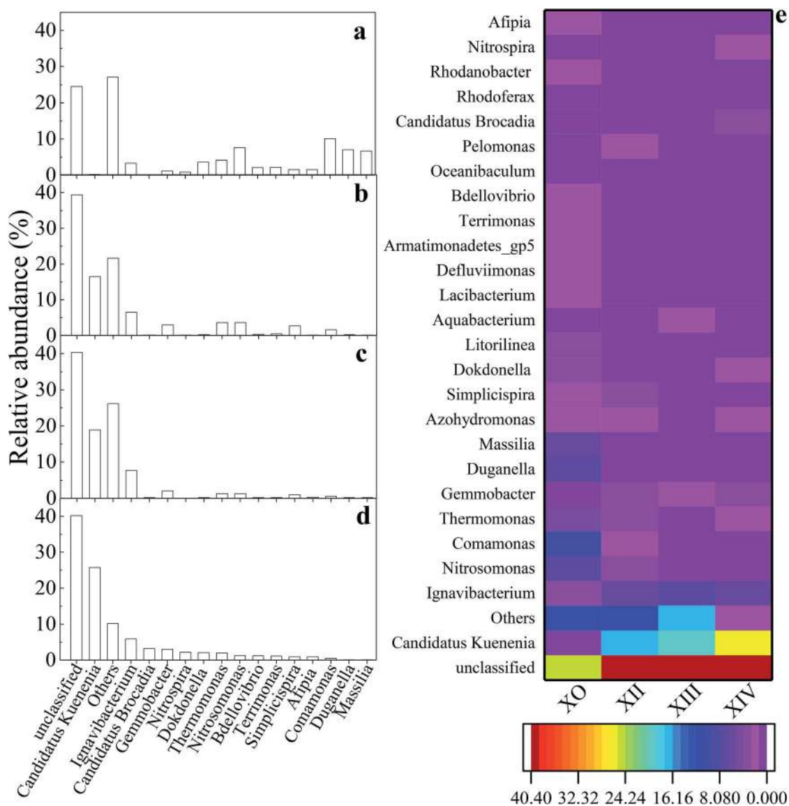
Fig. 5 Distribution of microbial community composition at the genus level (sequence reads \geq 1\% ): (a) X_0 ; (b) X_{II} ; (c) X_{III} ; (d) X_{IV} ; (e) richness heatmap depicting top 26 predominant genera within inoculum and reactor sludge samples.
