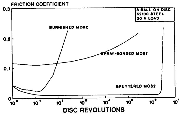
Figure 2-1. Friction Coefficient of MoS 2 Films Deposited by Various Techniques. From [10].
