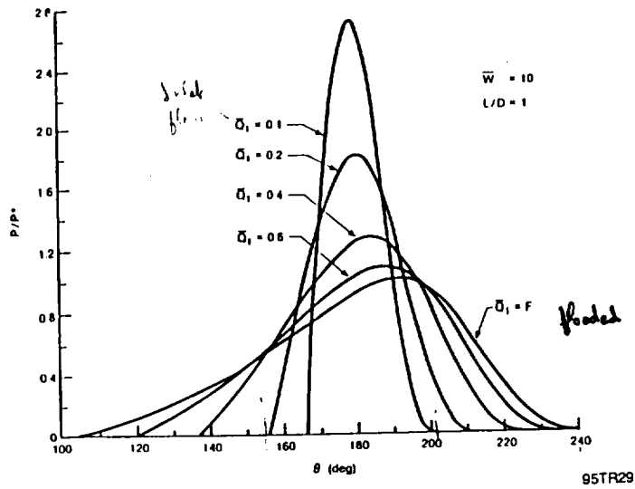
Figure 3-11. Pressure Profile at Bearing Midplane for Various Degrees of Starvation. From [10].
