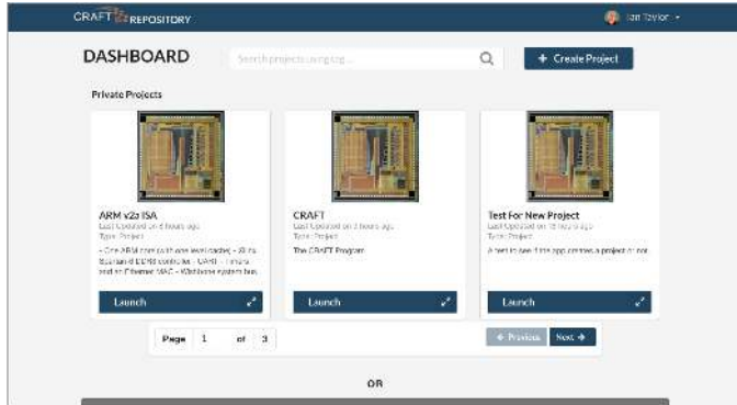
Fig. 3. CRAFT main dashboard screen.
