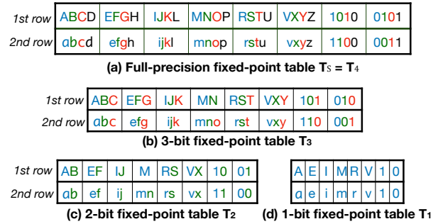
Figure 1: Four fixed-point quantized tables ( T_4 , T_3 , T_2 , T_1 ) containing 2 data points with 8 features. Each table has two rows and eight columns, and each element has four bits, where the symbol (e.g., A-Z, a-z) is binary, 0 or 1.
