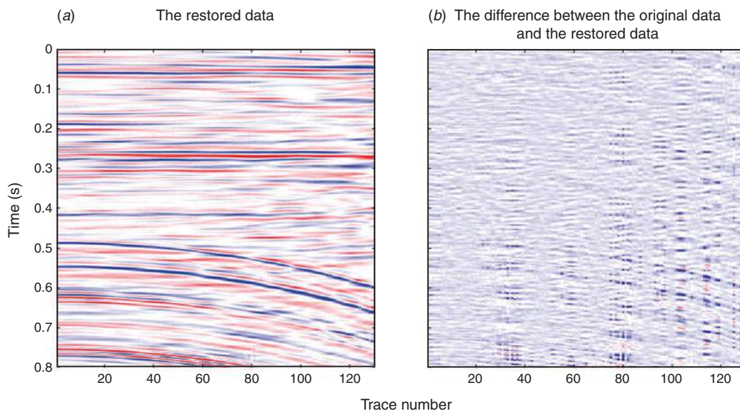
Fig. 11. (a) Interpolation of poststack data by SPGL1 method. (b) Difference between (a) and original poststack data.
