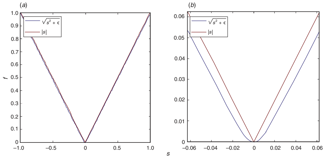
Fig. 1. (a) f_{\epsilon}(s) with \epsilon=0.0001 . (b) Magnified view of (a).
