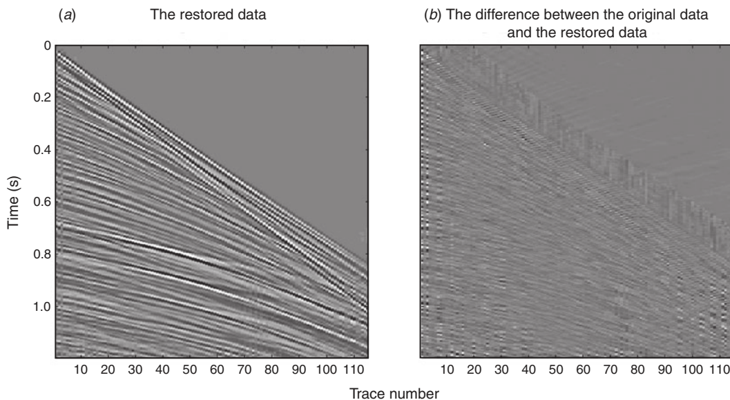
Fig. 7. (a) Interpolation of shot data by SPGL1 method. (b) Difference between (a) and original shot data.
