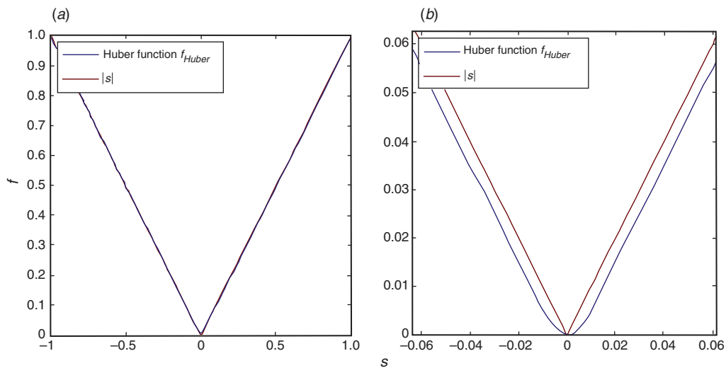
Fig. 3. (a) f_{Huber}(s) with a=0.0001 . (b) Magnified view of (a).
