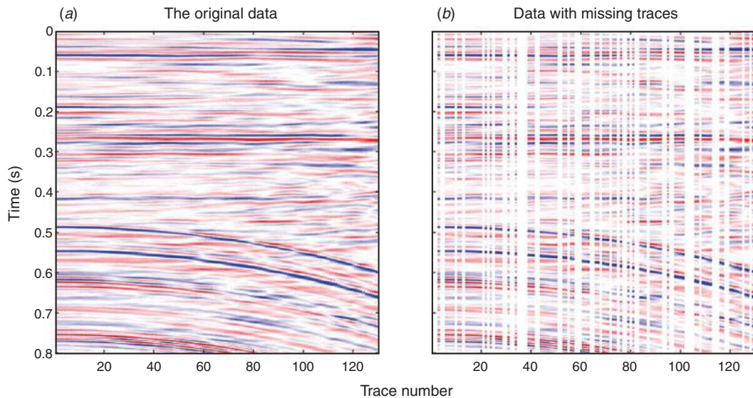
Fig. 8. (a) Original poststack data. (b) Sampled poststack data.
