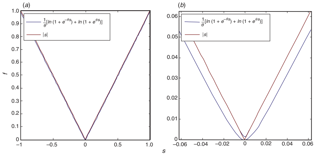
Fig. 2. (a) f_{\theta}(x) with \theta=10000 . (b) Magnified view of (a).
