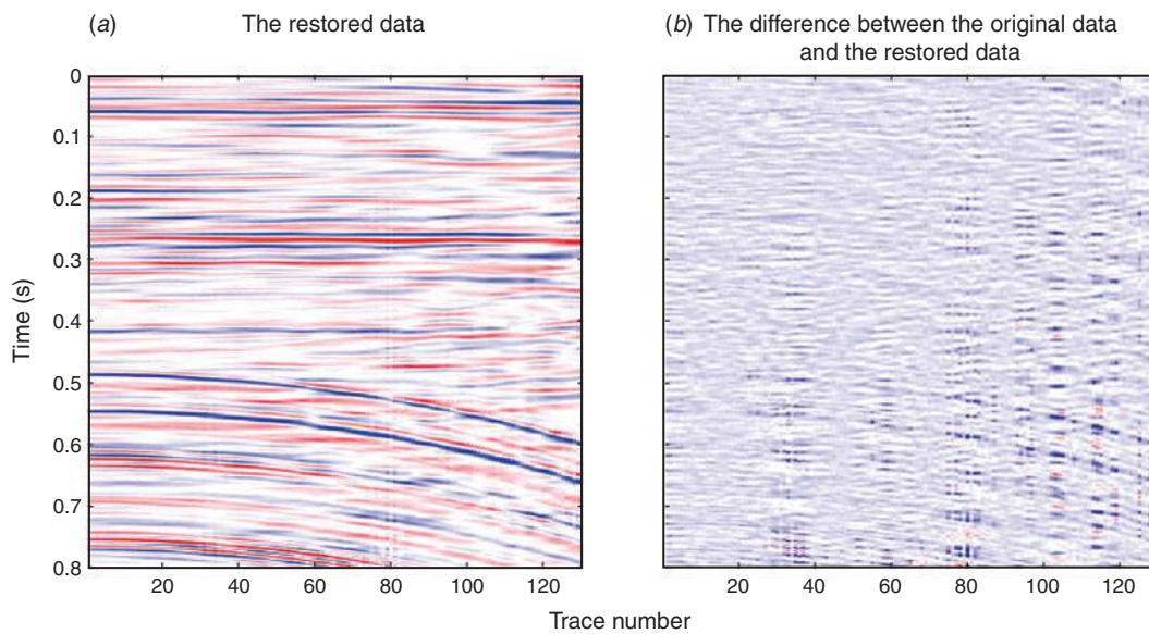
Fig. 10. (a) Interpolation of poststack data by FISTA method. (b) Difference between (a) and original poststack data.
