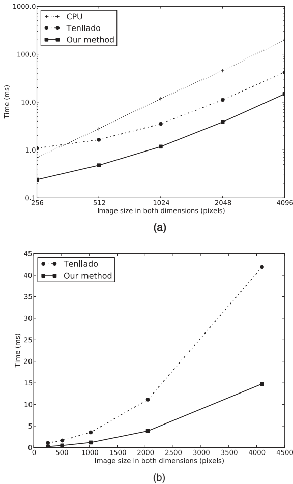
Fig. 9. Computation time versus image size for various lifting implementations; three-level Daubechies (9,7) forward transform. (a) The Schrödinger CPU implementation [12] and our CUDA-accelerated method in a log-log plot. (b) Just the two GPU methods in a linear plot.
