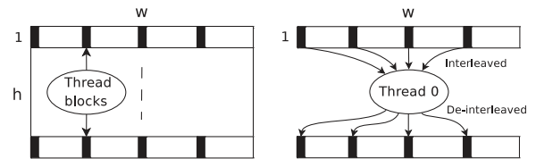
Fig. 4. Horizontal lifting step. h thread blocks are created, each containing T threads; each thread performs computations on N/(hT) = w/T data. Black quads illustrate input for the thread with id 0. Here, w and h are the dimensions of the input and N = w \cdot h .
