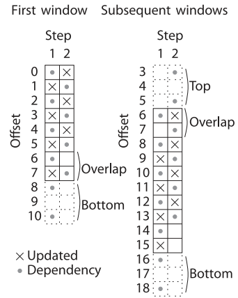
Fig. 8. The vertical pass for the Deslauriers-Dubuc (13, 7) [22] wavelet. Lifted rows in each step are marked with a cross, and dependent rows are marked with a bullet.
