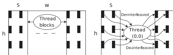
Fig. 6. Vertical lifting step. w/S blocks are created, each containing T = V_x \cdot V_y threads; each thread performs computations on S/V_x \times h/V_y data. Black quads illustrate input for the thread with id (0, 0) , whereas vertical lines depict boundaries between image-high slabs.
