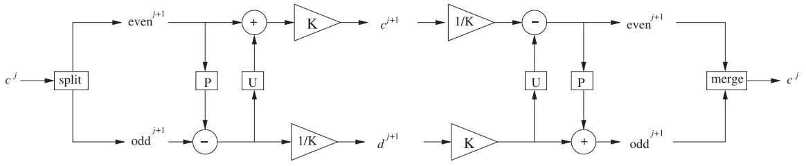
Fig. 3. Classical lifting scheme (one stage only). Left part: forward lifting. Right part: inverse lifting. Here, “split” is the trivial wavelet transform, “merge” is the opposite operation, P is the prediction step, U the update step, and K the scaling factor.
