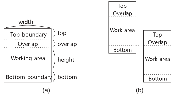
Fig. 7. (a) The sliding window used during the vertical pass for separable wavelets. (b) Advancing the sliding window: the next window is aligned at the bottom of the previous one, taking the overlap area into account.
