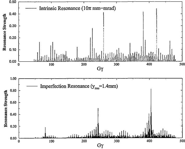
FIGURE 1. RHC spin resonance spectrum. The top plot is for the intrinsic resonances and the bottom plot is for imperfection resonances. A lattice of RHC 2000 polarized proton commissioning was used.
