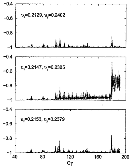
FIGURE 6. Spin tracking results for strongly coupled Blue ring with an emittance of 25 \pi mm-mrad and \nu_{rms}=0.6 mm. The three plots show polarization versus G\gamma with the fractional part of horizontal betatron tune near 3/14. The middle plot shows depolarization due to the coupling snake resonance at 3/14.
