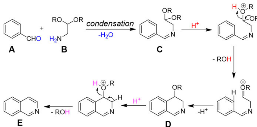
Scheme 1. The plausible mechanism of Pomeranz–Fritsch reaction.
