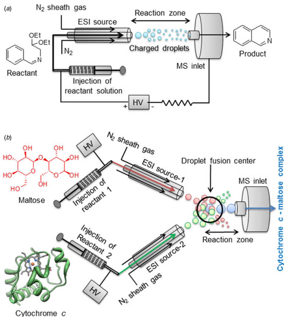
Fig. 1. Schematic diagrams of the experimental setup used in our study of ‘microdroplet chemistry’. The upper panel (a) shows the electropray assisted synthesis of isoquinoline, and the lower panel (b) shows the droplet fusion mass spectrometry to study the complexation between maltose and cytochrome c .
