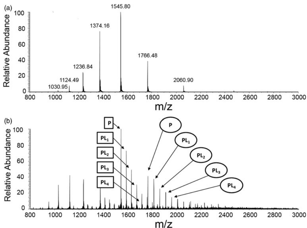
Fig. 3. ESI-mass spectra of (a) cytochrome c (100 \mu\text{M} ) and (b) cytochrome c (100 \mu\text{M} ) incubated with maltose (100 mM) for 20 min. The subscript n in \text{PL}_n denotes the number of bound maltose to cytochrome c (square denotes +8 charge state and circle denotes +7 charge state).
