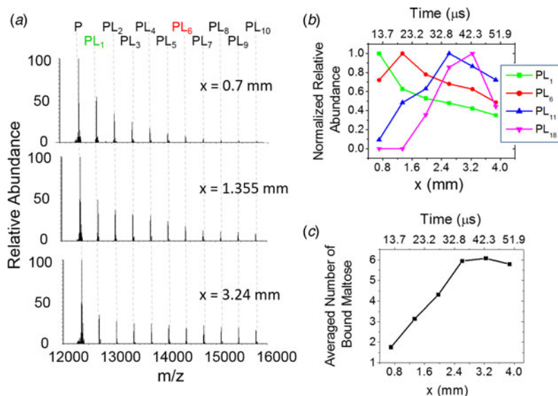
Fig. 4. Kinetics of the binding of cytochrome c and maltose. (a) Deconvoluted mass spectra at different distances ( x ) with cytochrome c (100 \mu\text{M} ) in one droplet source and maltose (100 mM) in the other source. The subscript n in \text{PL}_n denotes the number of maltose bound to cytochrome c . (b) Normalized relative abundances of cytochrome c with different number of bound maltose (green square: \text{PL}_1 , red circle: \text{PL}_6 , blue triangle up: \text{PL}_{11} , magenta triangle down: \text{PL}_{18} ). The normalized factor for each plot for \text{PL}_1 , \text{PL}_6 , \text{PL}_{11} , and \text{PL}_{18} is \times 1 , \times 4.7 , \times 11.7 , and \times 17.4 , respectively. (c) Average number of bound maltose to cytochrome c as a function of distance x and reaction time. The axes on top of (a) and (c) show the converted reaction time from the corresponding distance.
