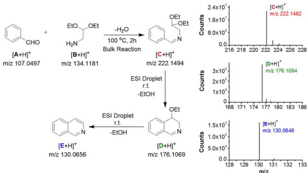
Fig. 2. Pomeranz–Fritsch synthesis of isoquinoline in the charged droplet produced by electrospray process. The left panel shows the two step synthesis of isoquinoline that we followed in the present study. In the first step, the conventional bulk reaction method was used to synthesize the precursor imine C. Then in the second step, the precursor C was injected from methanolic solution through an on-axis electrospray source, in positive ion mode, to form charged droplets encapsulating the precursor C, which was then converted into isoquinoline (E) inside the charged droplet via intermediate D. Each protonated species (precursor C, intermediate D, and product E) were detected and characterized by a high-resolution orbitrap mass spectrometer (see the spectra in the right panel; solvent: methanol). The theoretical values of m/z (see left panel) are in good agreement with that experimentally observed (see the right panel).
