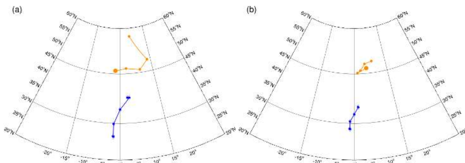
Figure 8. Track of the composite tropical cyclone (blue) and the downstream 500-hPa extratropical ridge (orange) from Day -2 to Day +2 for (a) rapid curvature acceleration, and (b) near-zero curvature acceleration. The composites are based on all TC tracks locations within 30–40°N. Day 0 is the reference day for the composites in Fig. 7
