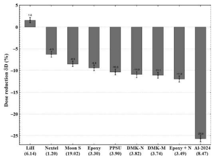
FIG. 9. Dose reduction of single materials exposed to 1,000 MeV/u 4 He ions. The target thicknesses in g cm -2 are reported in parentheses while the exact δD values are indicated in percentage on top of each column. The characteristics of all materials are shown in Table 1.
