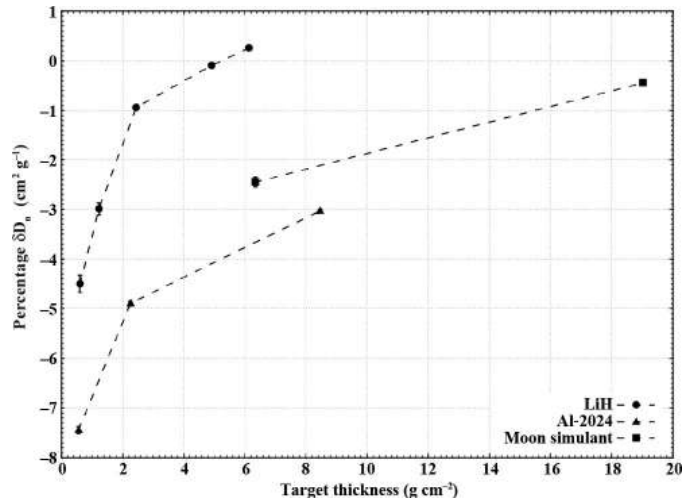
FIG. 8. Normalized dose reduction δD n as a function of depth for several material types exposed to 1,000 MeV/u 4 He ions. The values were calculated using Eq. (2). The characteristics of all materials are shown in Table 1.
