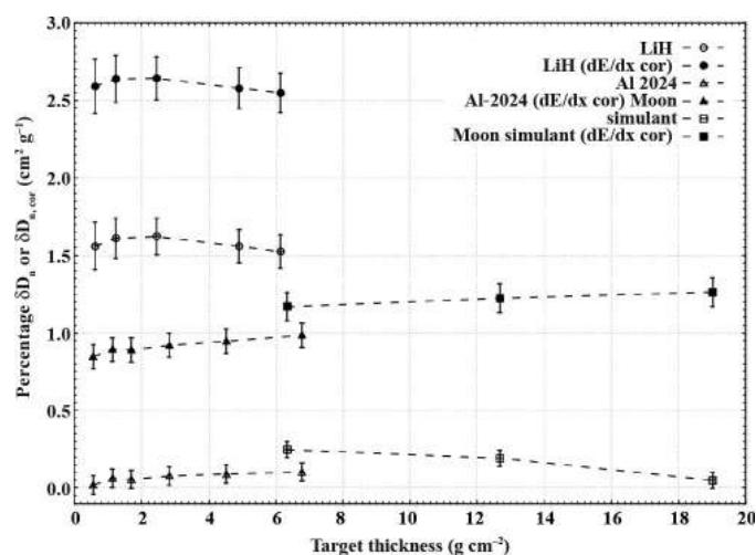
FIG. 6. Normalized dose reduction without (open symbols) and with (solid symbols) the energy loss correction as function of thickness for single shielding materials exposed to 430 MeV/u ^{12}\text{C} ions. The characteristics of all materials are shown in Table 1.
