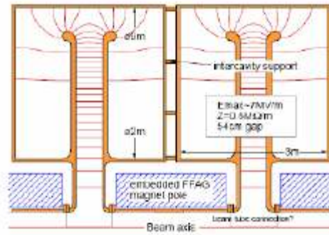
Fig. 21. 5 MHz vacuum cavity for FFAg scheme.
