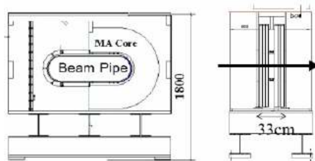
Fig. 22. 5 MHz ferrite-loaded cavity for FFAg scheme.
