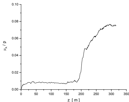
Fig. 31. Number of muons per incident proton accepted by the downstream acceleration system vs. longitudinal position along the ISS front end.
