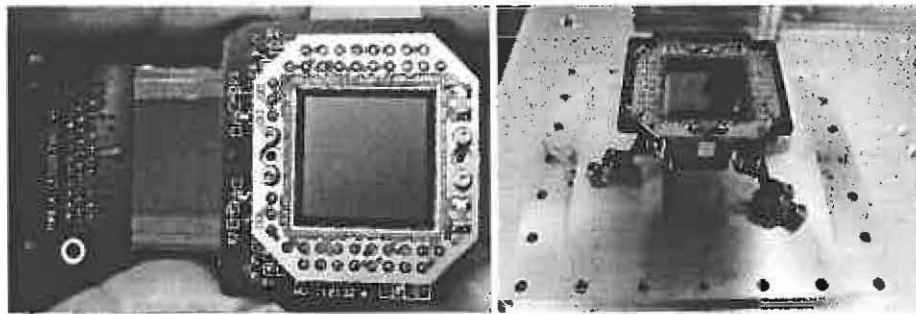
Figure 7. Left: Flex circuit design of detector electronics at focal plane. Right: Top view of detector with flight mount post vibration testing with launch loads.
