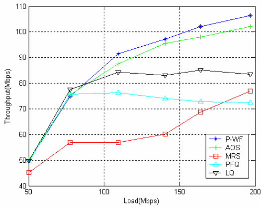
Figure 4: Performance of schedulers with varying load
