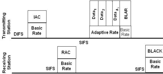
Figure 1: Example aggregate frame transmission
