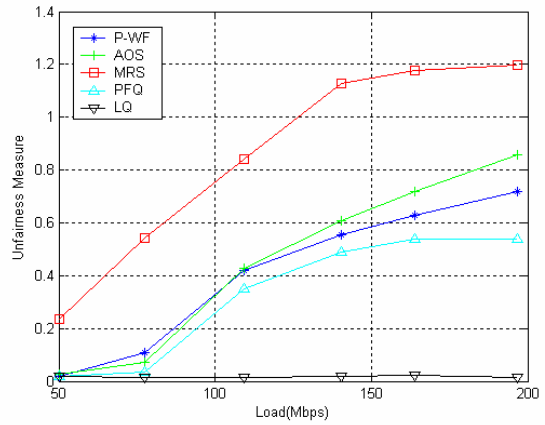
Figure 6: Fairness performance of proposed and existing schedulers
