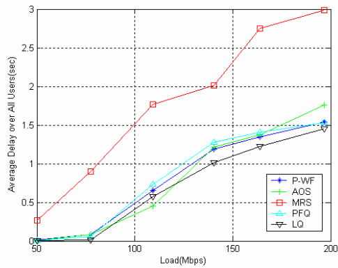
Figure 5: Mean user delay vs load.
