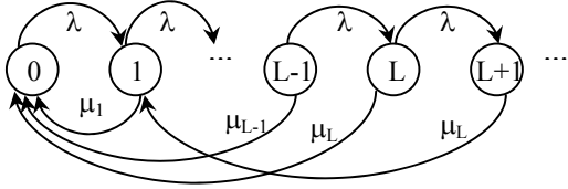
Figure 3: Markov-chain representation of aggregate frame transmission
