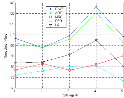
Figure 7: Performance of the schedulers with different topologies
