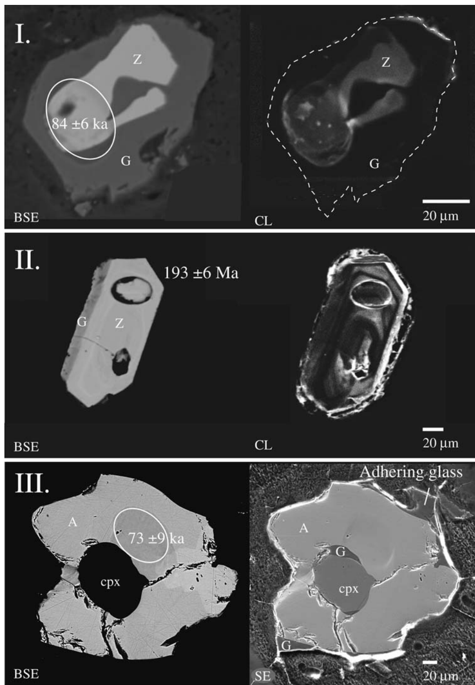
Fig. 3 Backscattered-electron ( BSE , left ) and cathodoluminescence or secondary electron ( CL/SE , right ) images of dated accessory minerals. I: Representative image of subhedral to anhedral Pleistocene zircon. II: Representative image of euhedral Mesozoic zircon. III: Representative image of subhedral to anhedral allanite. A allanite, G glass, Z zircon, cpx clinopyroxene
