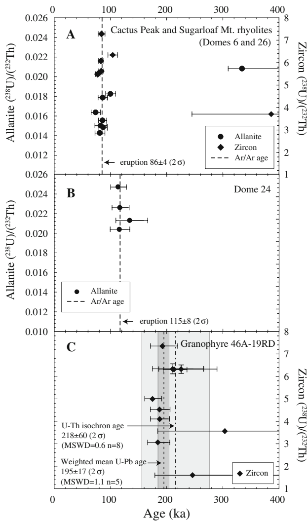
Fig. 4 ^{238}\text{U} – ^{230}\text{Th} ages and (^{238}\text{U})/(^{232}\text{Th}) compositions for allanite and zircon from selected Coso rhyolites. a Cactus Peak and Sugarloaf Mt. rhyolites, b Dome 24, and c Granophyre drill core 46A-19RD. Symbols are defined in figure. Uncertainty of ion microprobe spot analyses are 1\sigma . ^{40}\text{Ar}/^{39}\text{Ar} eruption ages (this study) included for reference. Vertical shaded bands show uncertainty for weighted mean ^{238}\text{U} – ^{206}\text{Pb} (dashed) and ^{238}\text{U} – ^{230}\text{Th} isochron (dot-dashed) ages for Pleistocene zircon from the granophyre
