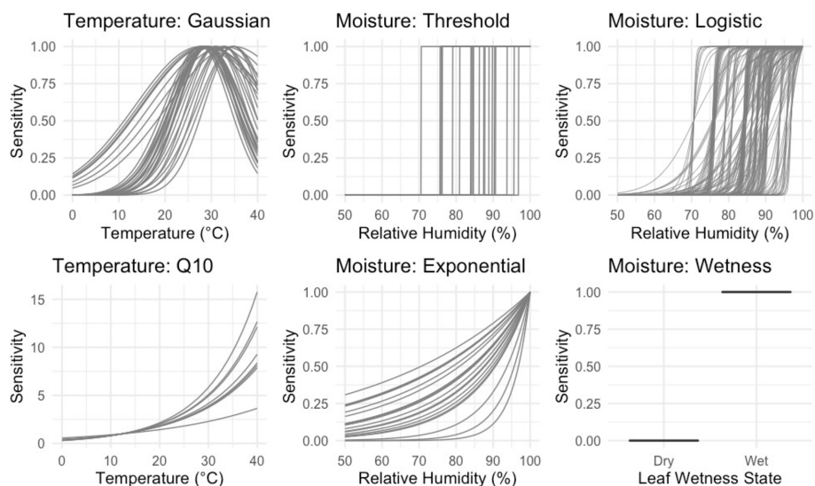
Figure 1. Temperature and NRM sensitivity functions included in the models. Each curve shows one parameter combination chosen by random sampling using a normal distribution around a specified set of priors as identified in Table 2 ( n = 895\,230 total combinations). The wetness moisture function has no parameter and is simply the proportion of time during each hour that the leaf wetness sensor detected the presence of moisture.
