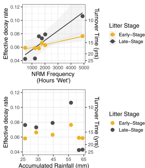
Figure 4. Effective decay rate calculated without explicit temperature or NRM sensitivity (Eq. 1) relative to NRM frequency and accumulated rainfall during the study period. Among sites, decay rate constant was strongly correlated with the proportion of time that a site experienced NRM conditions (early-stage: R^2 = 0.87 , P = 0.007 , slope = 4.311 \times 10^{-6} ; late-stage: R^2 = 0.80 , P = 0.02 , slope = 1.421 \times 10^{-5} ) but was uncorrelated with total rainfall (early-stage: R^2 = 0.01 , P = 0.87 ; late-stage: R^2 = 0.14 , P = 0.46 ).
