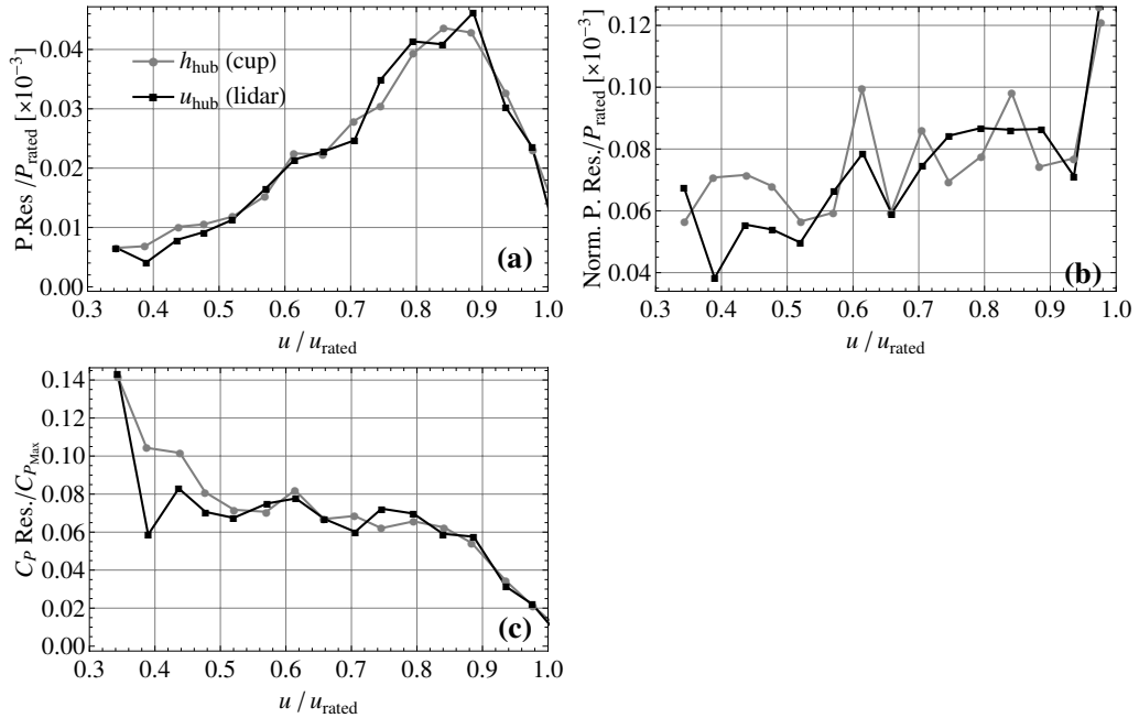
Figure 8.4: (a): Mean residual in the power curve ( P. Res. ); (b): Normalized residual in the power curve ( Norm. P. Res. ); (c): Mean residual in the C_P curve ( C_P Res. )
