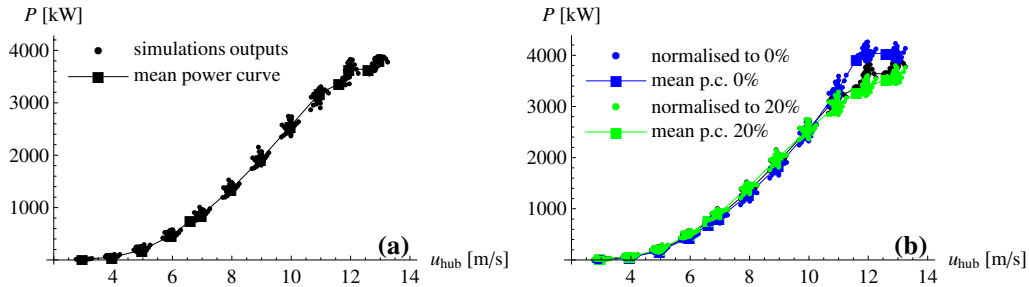
Figure 5.6: (a): Power curve scatter plot obtained with the output of the simulations cases with various turbulence intensities between 5% and 20% and no shear; (b): Results of the normalisation of the power curve shown in(a) to 0% and 20% turbulence intensity with Albers' method
