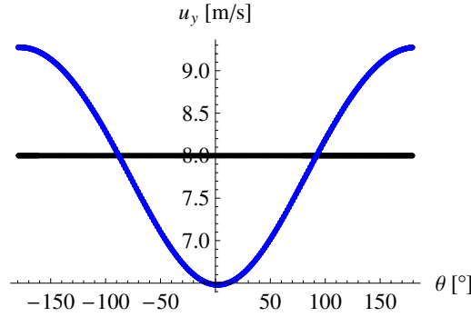
Figure 3.4: Free wind speed seen from a rotating point, positioned at a radius of 30m, as a function of the azimuth angle. Black: no shear; Blue: power law profile with shear exponent of 0.5. (0° corresponds to downwards)
