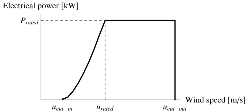
Figure 1.1: Typical wind turbine power curve
