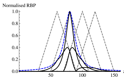
Figure 6.5: Weighting of the backscatter for a pulsed focused lidar.
