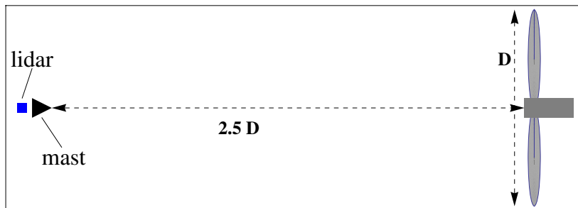
Figure 8.1: Sketch of the experimental set up
