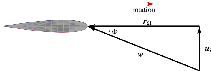
Figure 3.5: Speed triangle for a blade element. \mathbf{u}_i is the induced wind speed, \mathbf{r}_\Omega the opposite of blade speed at this radius, \mathbf{w} the relative speed and \Phi the angle between the rotor plane and \mathbf{w} corresponding to the sum of the pitch angle, the twist angle and the angle of attack.
