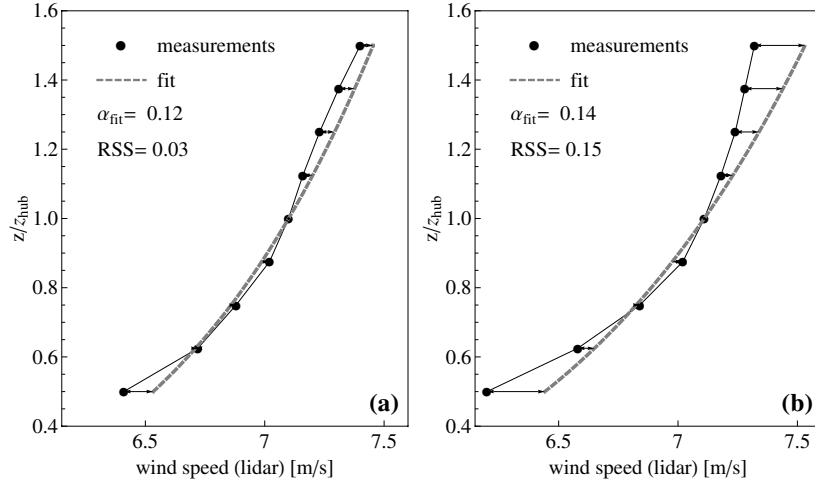
Figure 8.5: Example of measured profiles and their fit to a power law profile; (a): RSS \leq 0.1 , (b): RSS > 0.1
