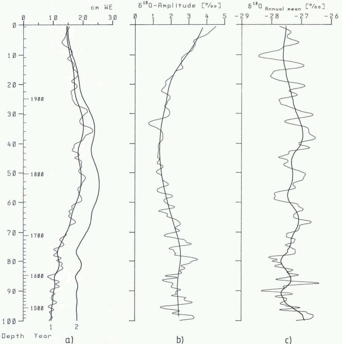
Fig. 7. Ice core T340, drilled in 1984 on Ronne Ice Shelf: (a) (1) thickness of the annual layers, (2) estimated accumulation rates corrected for creep thinning, both versus depth and/or time of deposition in centimetres water equivalent; (b) annual amplitude of the ^{18}\text{O} content; (c) mean annual ^{18}\text{O} content after subtraction of the linear trend ( \delta^{18}\text{O} = -27.3 - 0.049z ). All the curves have been smoothed by filtering techniques.
