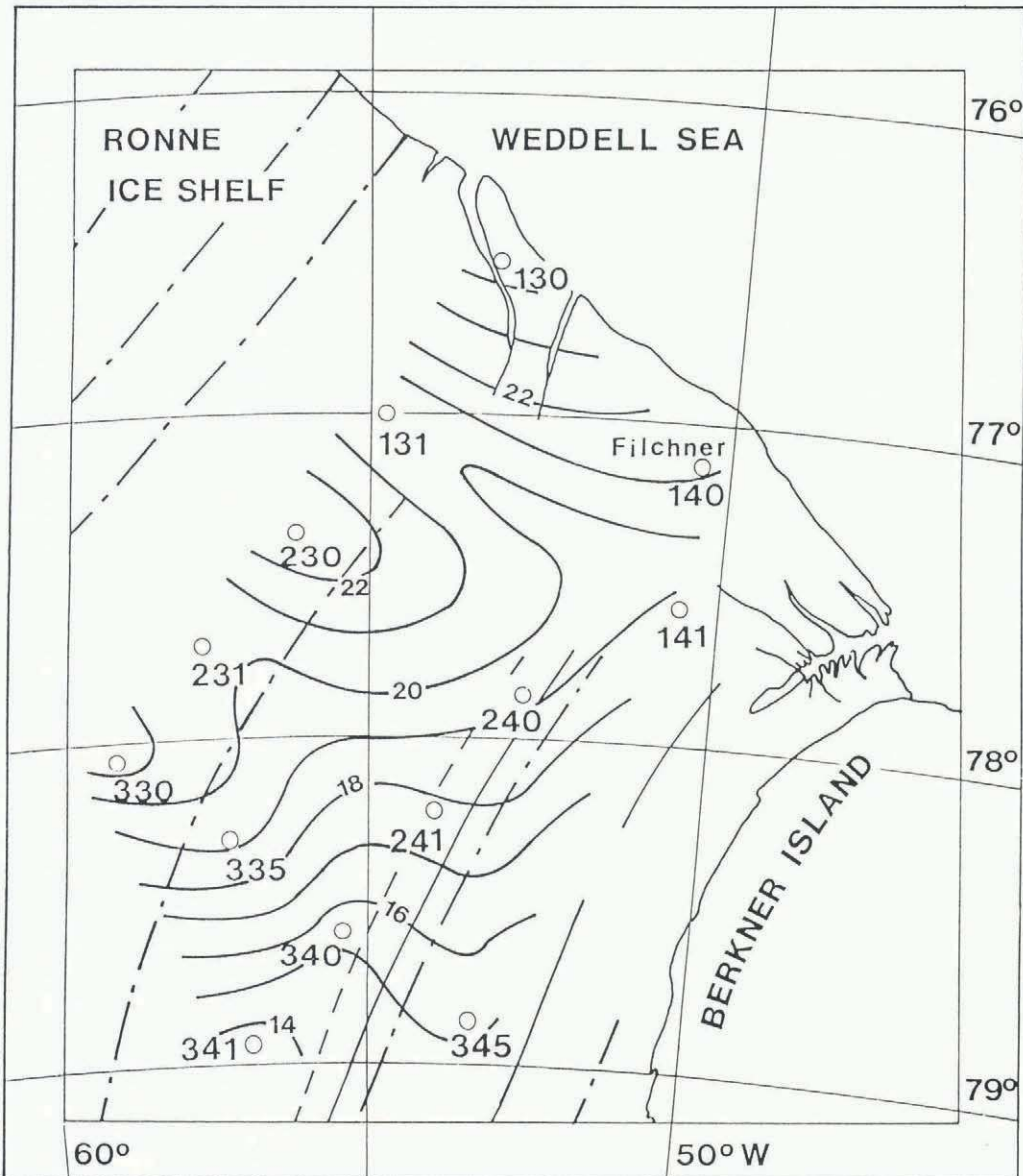
Fig. 5. Distribution of the accumulation rates in the eastern part of Ronne Ice Shelf. Isolines of accumulation are plotted at intervals of 1 \text{ g cm}^{-2} \text{ a}^{-1} .
