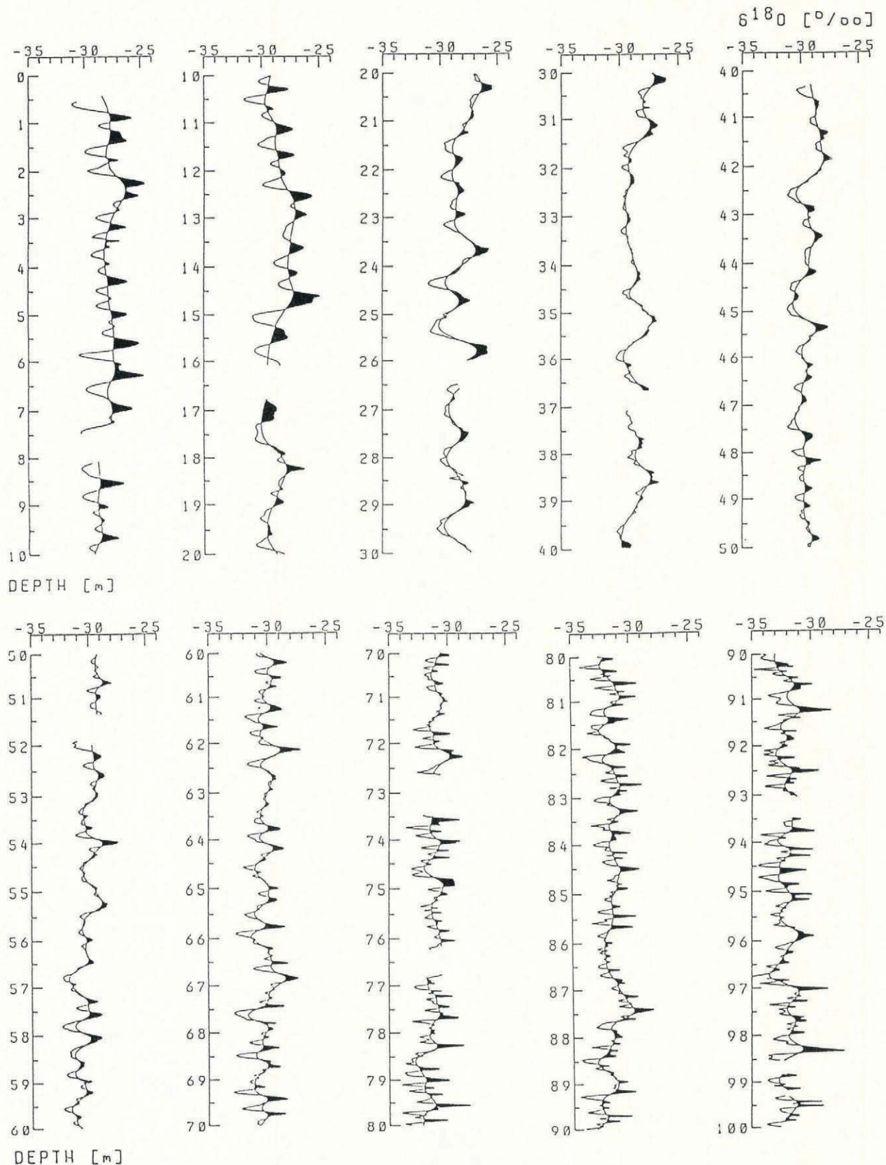
Fig. 6. ^{18}\text{O} profile of ice core T340, drilled in 1984 at point 340 on Ronne Ice Shelf (Fig. 1). Material originating from summer precipitation is dark-coloured. The base line represents the variation in the annual ^{18}\text{O} content.
