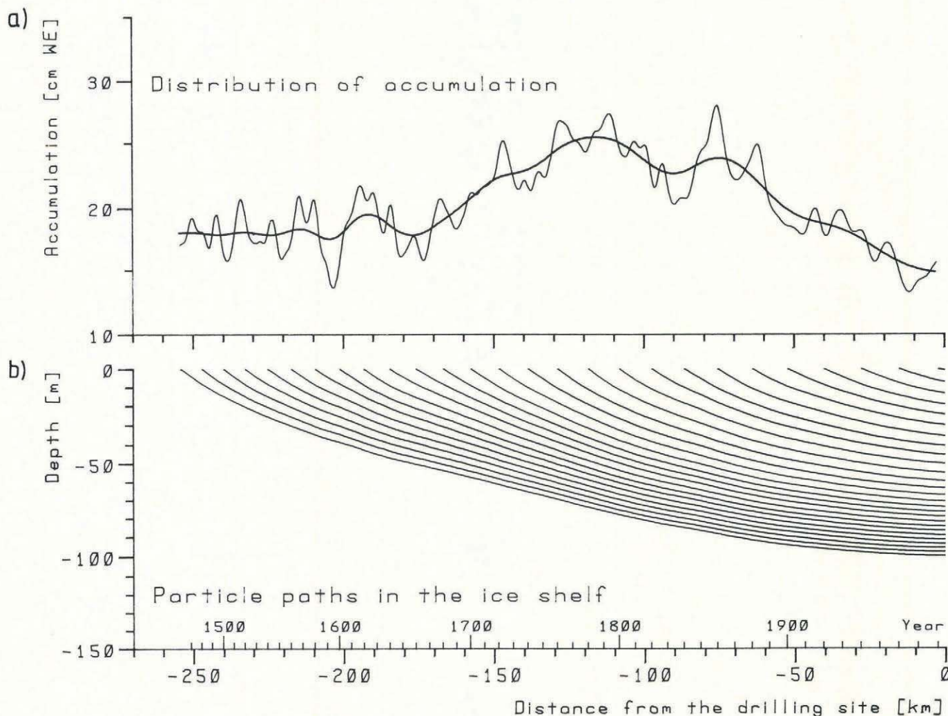
Fig. 8. Ice core T340, drilled in 1984 on Ronne Ice Shelf: (a) distribution of the accumulation rate up-stream of the drilling site, which fits the layer sequence found in the ice core; (b) particle paths to the bore hole.
