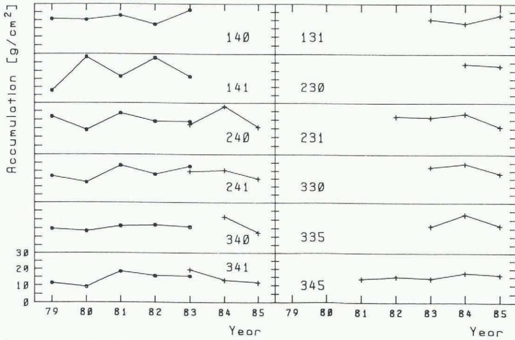
Fig. 4. Amount of annual accumulation at the measuring points of the Filchner I and Filchner II field programmes. (o) snow-pit 1984; (+) snow-pit 1986.
