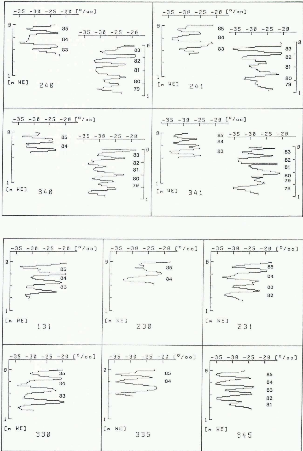
Fig. 2. Profiles of the ^{18}\text{O} content of snow-pits at measuring points of the 1983-84 and 1985-86 field seasons (Fig. 1). The profiles of the snow-pits dug in 1984 are dislocated by the amount of the previous year's accumulation, so that corresponding years are displayed at the same level.
