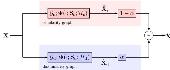
Fig. 2. Rating prediction with similar and dissimilar Graphs. We construct a NN graph \mathcal{S}_s capturing similarities between entities, and a FN graph \mathcal{S}_d capturing dissimilarities between entities. On each graph, we run a graph convolutional module \Phi(\cdot) with respective parameter set \mathcal{H}_{(\cdot)} [cf. (4), (9)]. The estimated outputs are combined through a parameter \alpha to obtain the final joint estimate \hat{X} .
