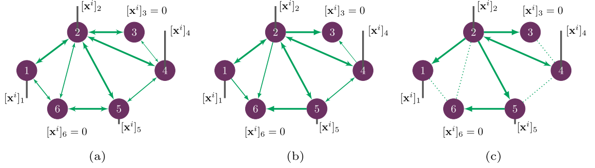
Fig. 1. Building an item-specific graph B_i from the global correlation graph B . (a) User graph B . Nodes represent users and arrows correlations. Ratings to item i are a graph signal x_i shown by vertical bars. (b) Treat each undirected edge as two directed edges. Remove any directed edge starting from a user who did not rate item i . (c) Keep the n = 1 strongest incoming edge for each user representing the nearest neighbor. The adjacency matrix of this graph is B_i .
