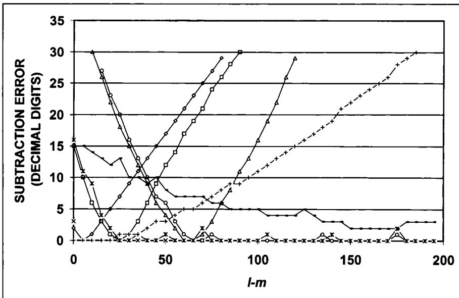
FIG. 2. Subtraction error in decimal digits obtained in the numerator of the traditional expression (8) plotted versus l - m for selected parameters (c, m, \xi) : \diamond(10, 0, 1.00000001) ; \times(10, 0, 10) ; +(10, 100, 1.01) ; \square(40, 0, 1.00000001) ; \star(40, 0, 10) ; \Delta(100, 0, 1.00000001) ; \circ(100, 0, 10) ; - (100, 100, 10)
