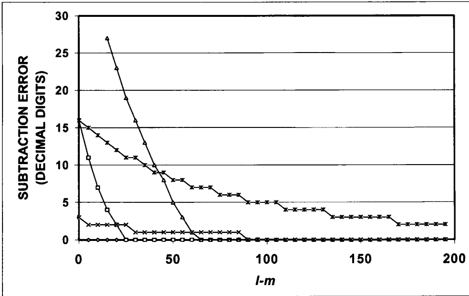
FIG. 1. Subtraction error in decimal digits obtained in the denominator of the traditional expression (8) plotted versus l-m for selected parameters (c, m) : \diamond(10, 0) ; \square(40, 0) ; \times(40, 100) ; \Delta(100, 0) ; \star(100, 100)
