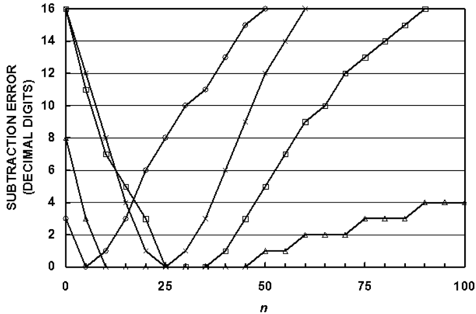
FIG. 2. Subtraction error in decimal digits in Mc_n^{(1)}(\xi, c) calculated using (11) plotted versus n for selected values of (\xi, c) : o (1.001, 10); x (1.001, 40); □ (1.1, 40); Δ (2, 20).
