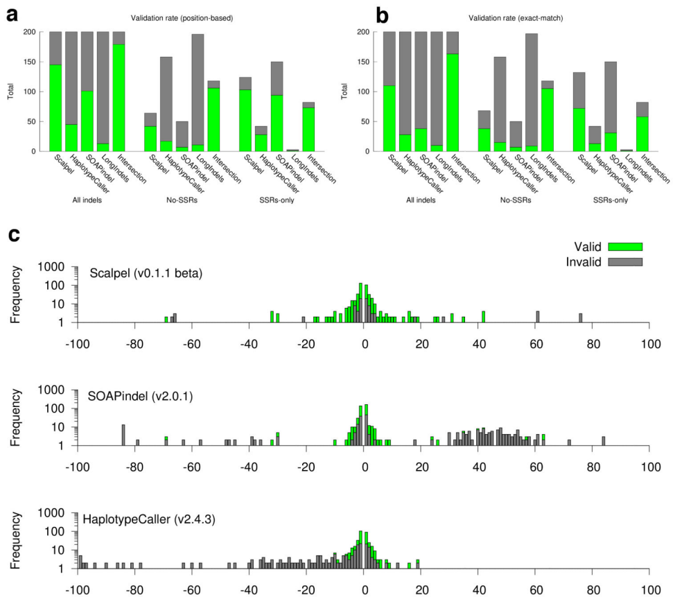
Figure 3. MiSeq validation
