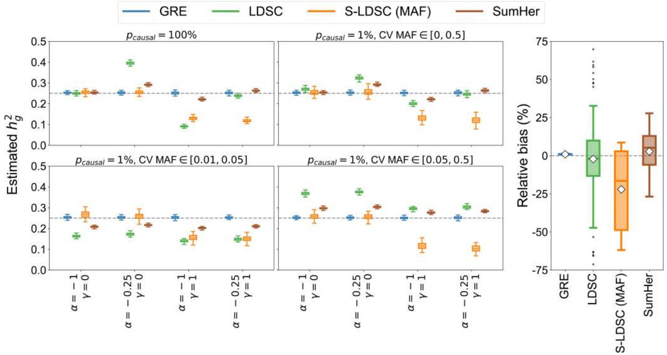
Figure 2. Comparison of \hat{h}_{GRE}^2 with LDSC, S-LDSC (MAF), and SumHer in genome-wide simulations ( N = 337205 , M = 593300 , h_g^2 = 0.25 ). Left: Phenotypes were drawn under one of 16 MAF- and/or LDK-LD-dependent architectures by varying p_{causal} , \alpha , \gamma , and CV MAF (Methods). Each boxplot contains estimates of h_g^2 from 100 simulations. Right: Relative bias of each method (as a percentage of h_g^2 ) across 112 distinct MAF- and LDK-LD-dependent architectures (Methods). Each boxplot contains 112 points; each point is the relative bias estimated from 100 simulations under a single genetic architecture. The white diamonds mark the average of each distribution. Boxplot whiskers extend to the minimum and maximum estimates located within 1.5 \times IQR from the first and third quartiles, respectively.
