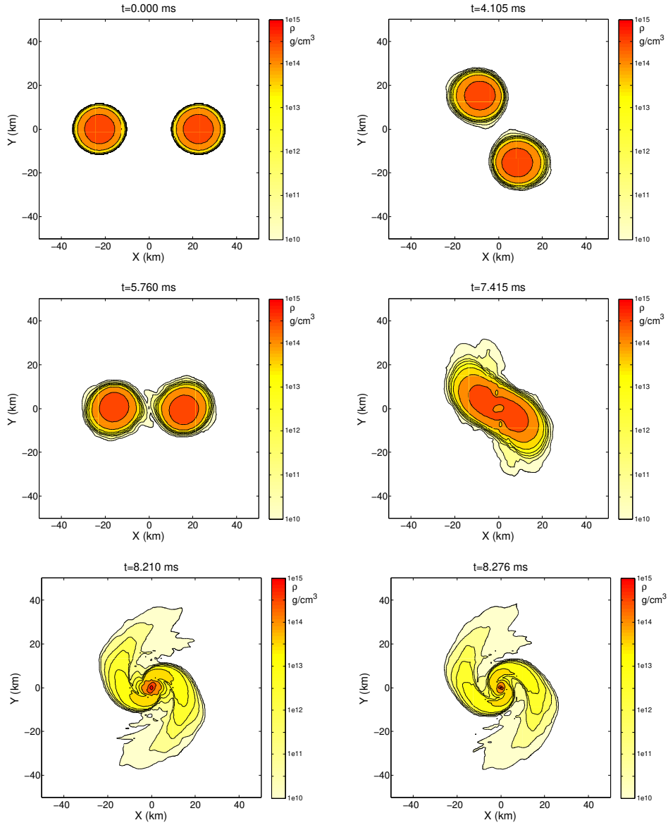
Figure 1. Isodensity contours for the M3 . 6q1 . 00 model on the (x, y) plane. The times when the frames have been taken are shown on top of the plots while the color-code for the rest-mass density is indicated to the right of each plot. Additionally, isodensity contours are shown for the values of \rho = 10^{10}, 10^{11}, 10^{12}, 10^{12.5}, 10^{13}, 10^{13.5}, 10^{14}, 10^{14.5}, 10^{15} \text{ g/cm}^3 . The third frame (at time t = 5.760 ms) shows the onset of the merger, the last two frames (at times t = 8.210 ms, t = 8.276 ms) show the behaviour of the system during the collapse to a BH.
