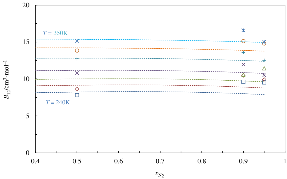
Fig. 8. The second interaction virial coefficient B_{12}(T) for the (N_2 + H_2) binary system estimated from the experimental data: □ T = 240\text{ K} ; ◇ T = 250\text{ K} ; △ T = 260\text{ K} ; × T = 275\text{ K} ; + T = 300\text{ K} ; ○ T = 325\text{ K} ; * T = 350\text{ K} . The dashed lines represent the B_{12}(T) values estimated from the GERG-2008 EoS at different temperatures.
