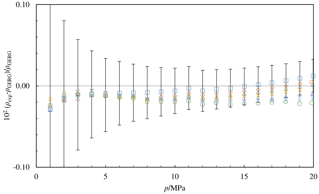
Fig. 1. Relative deviations in density of experimental ( p, \rho, T ) data of the (0.94999954 N 2 + 0.05000022 H 2 ) mixture \rho_{\text{exp}} from density values calculated from the GERG-2008 equation of state \rho_{\text{GERG}} versus pressure: \square T = 240 K; \diamond T = 250 K; \triangle T = 260 K; \times T = 275 K; + T = 300 K; \circ T = 325 K; * T = 350 K. Error bars on the 240 K isotherm indicate the expanded uncertainty ( k = 2 ) of the experimental density data calculated with Eq. (4).
