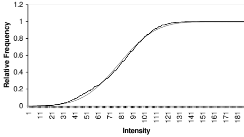
Fig. 3 Comparison between cumulative distribution of a normal distribution and a cumulative distribution of intensity of an iris image. The gray and black curves represent the normal and iris's distribution respectively. Their means and standard deviations are same.
