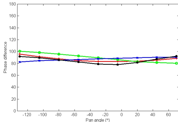
Fig. 8. The phase difference of four different orientations along an arc generated by panning the tag.
