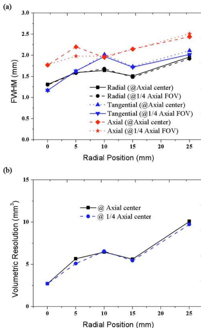
FIG. 5. (a) Simulated spatial resolution of the X-PET™ scanner in terms of FWHM according to NEMA NU-4 standards. (b) Resulting volumetric spatial resolution obtained by multiplication of radial, tangential, and axial FWHMs.
