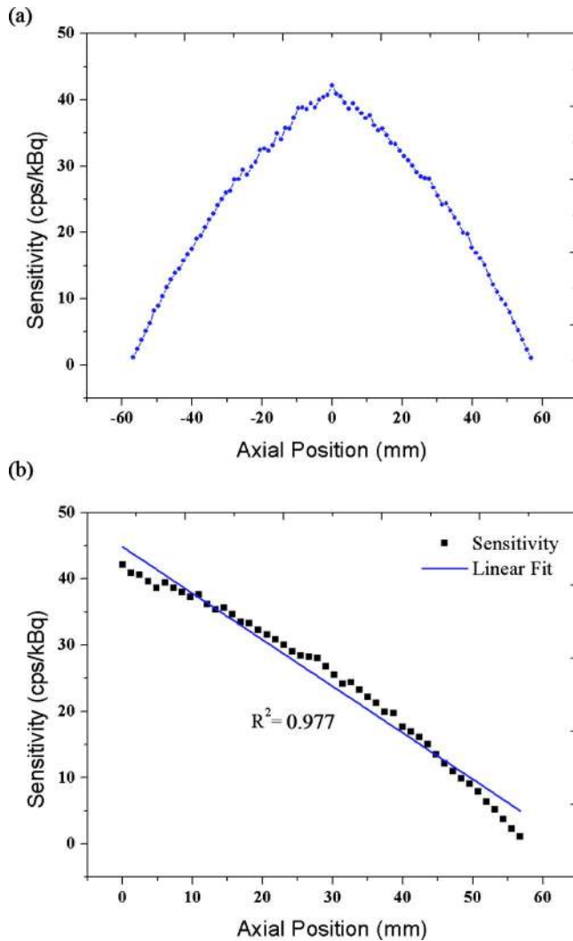
FIG. 6. (a) Sensitivity profile of the X-PET TM scanner over axial positions calculated according to NEMA NU-4 2008 standards. (b) Homogeneity of the sensitivity profile along the axial direction.
