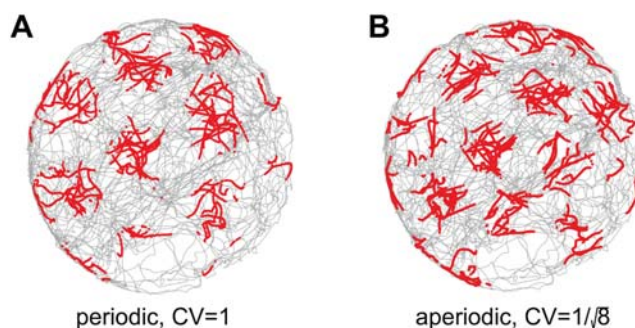
Figure 5. Single neuron (SN) responses from stochastic spiking networks. (A) SN response in a stochastic spiking periodic network. The parameters and input velocity trajectory are as in Figure 2A–C, except that spiking is simulated explicitly and the spikes are generated by an inhomogeneous Poisson process. (B) SN response in a stochastic spiking aperiodic network. The parameters are as in Figure 2D–F, except that spiking is simulated explicitly and the spikes are generated by a point process with a CV of 1/\sqrt{8} (see Methods ). Each red dot represents a spike.
