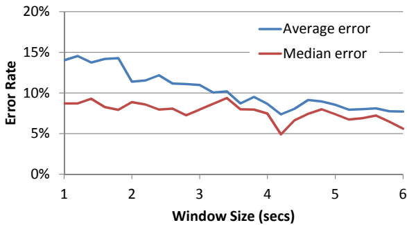
Figure 18: Error rates for speed calculations as a function of window size.
