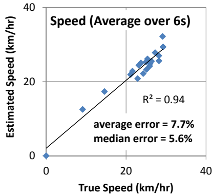
Figure 17: Correlation between calculated and true speed values for 6s windows of traffic footage.
