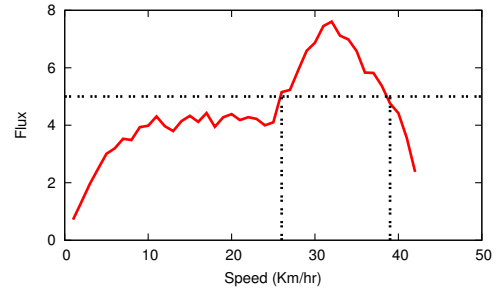
Figure 22: Flux vs. speed (based on 30s moving averages).
