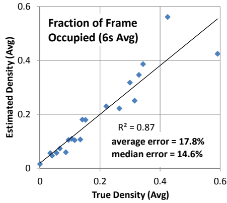
Figure 12: Correlation between calculated and true density values for 6s windows of traffic footage.
