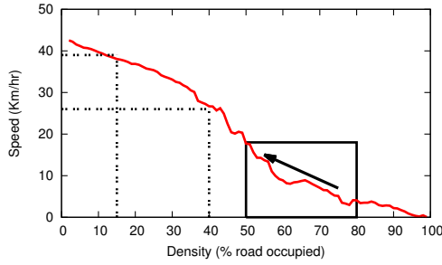
Figure 21: Speed vs. density (based on 30s moving averages).
