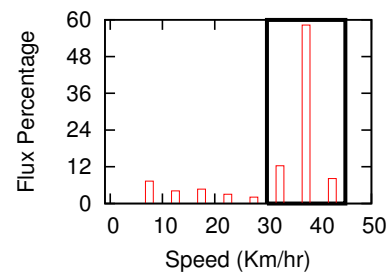
Figure 25: For 30s windows with flux between 4.5 - 5.5 on July 10, percentage of total flux that exhibited given speeds.
