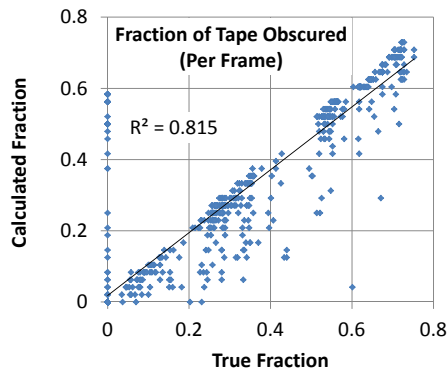
Figure 10: Comparison of frame-level density calculations with ground-truth values. Density estimates represent raw values (line 5 of algorithm), prior to correction.
