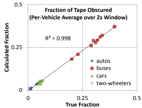
Figure 11: Comparison of vehicle-level density calculations with ground-truth values. Density estimates represent raw values (line 5 of algorithm), prior to correction.
