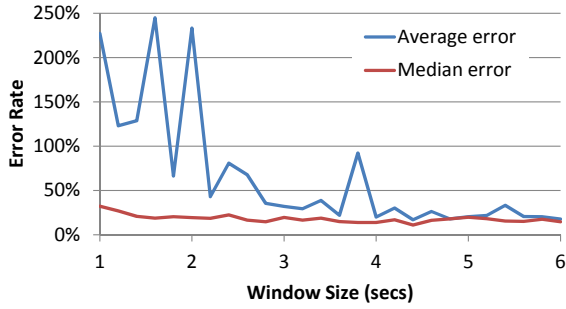
Figure 13: Density errors as a function of window size.
