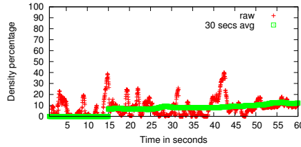
Figure 7: Background subtraction does not detect the buses in video excerpt.
