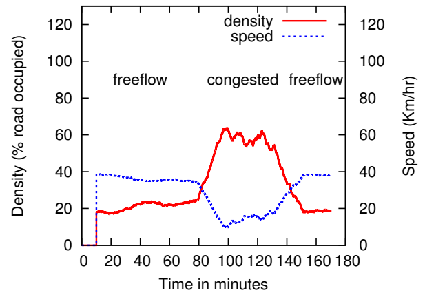
Figure 19: Traffic density and speed (20-minute moving average) from 8:15am to 11:15am on July 10.
