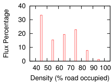
Figure 23: For 30s windows during congested periods on July 10, percentage of flux that exhibited given densities.
