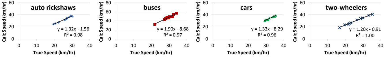
Figure 15: Correlation between calculated and true speed values for individual vehicle types.
