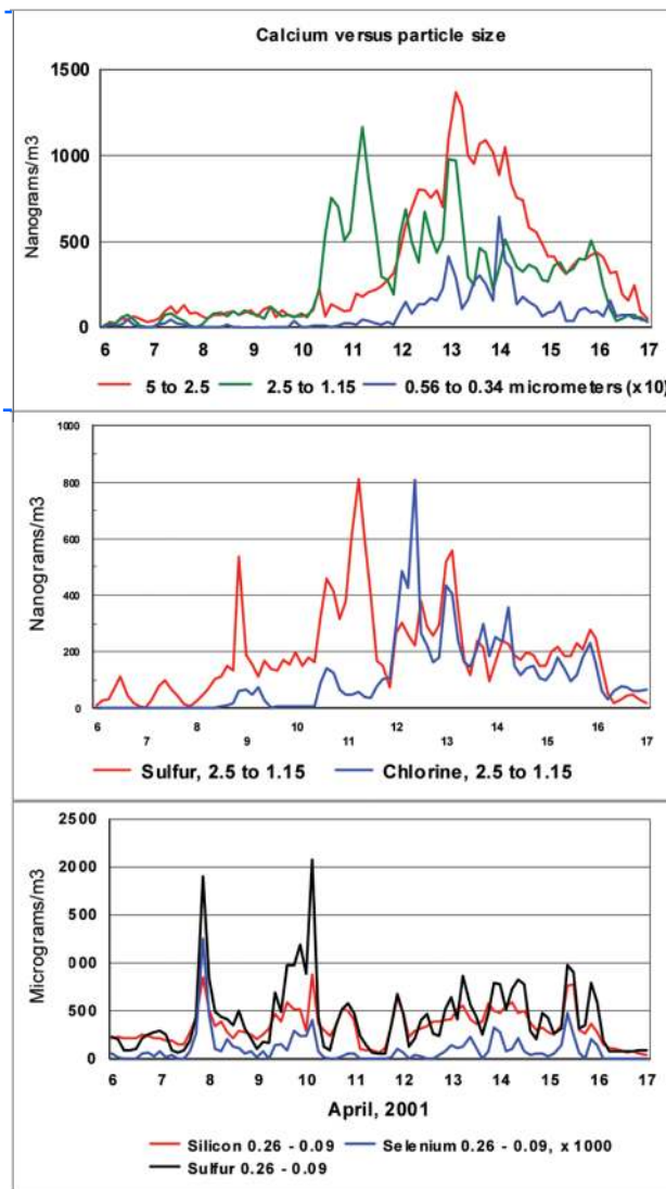
FIG. 7. Aerosol composition measured in several of the eight size ranges at the Tango site on the north coast of Japan. Air trajectory analyses show that five major source regions contributed to the observed data: 6–9 Apr slow trajectories over the Japanese inland sea; 10–11 Apr, same as the previous case plus the erupting volcano on Miyakejima, south of Tokyo; 12 Apr, a fast trajectory (6000 km in 4 days) from Siberia over the Taklimakan Desert in western China, and then over much of northern China; 13–14 Apr, somewhat slower trajectories from the Gobi Desert over Manchuria and Korea; and 15–16 Apr, slow trajectories from Beijing and Qingdao. (top) Calcium in three size modes, with the smallest size mode multiplied by 10. (middle) Calcium closely associated with sulfur in the same size mode, with relatively little silicon is a fingerprint for the Miyakejima volcano. The sharp increase in chlorine on 12 Apr resulted from sea salt NaCl transported in the high-wind regime to the site 6 km inland. Gobi dust arrived with anthropogenic elements and the highest accumulation mode sulfur seen in the entire 42-day experiment. (bottom) Highly correlated elements in the very fine mode ( 0.29 – 0.09 \mu\text{m} ) previously seen in studies of coal-fired power plants in the western United States.
