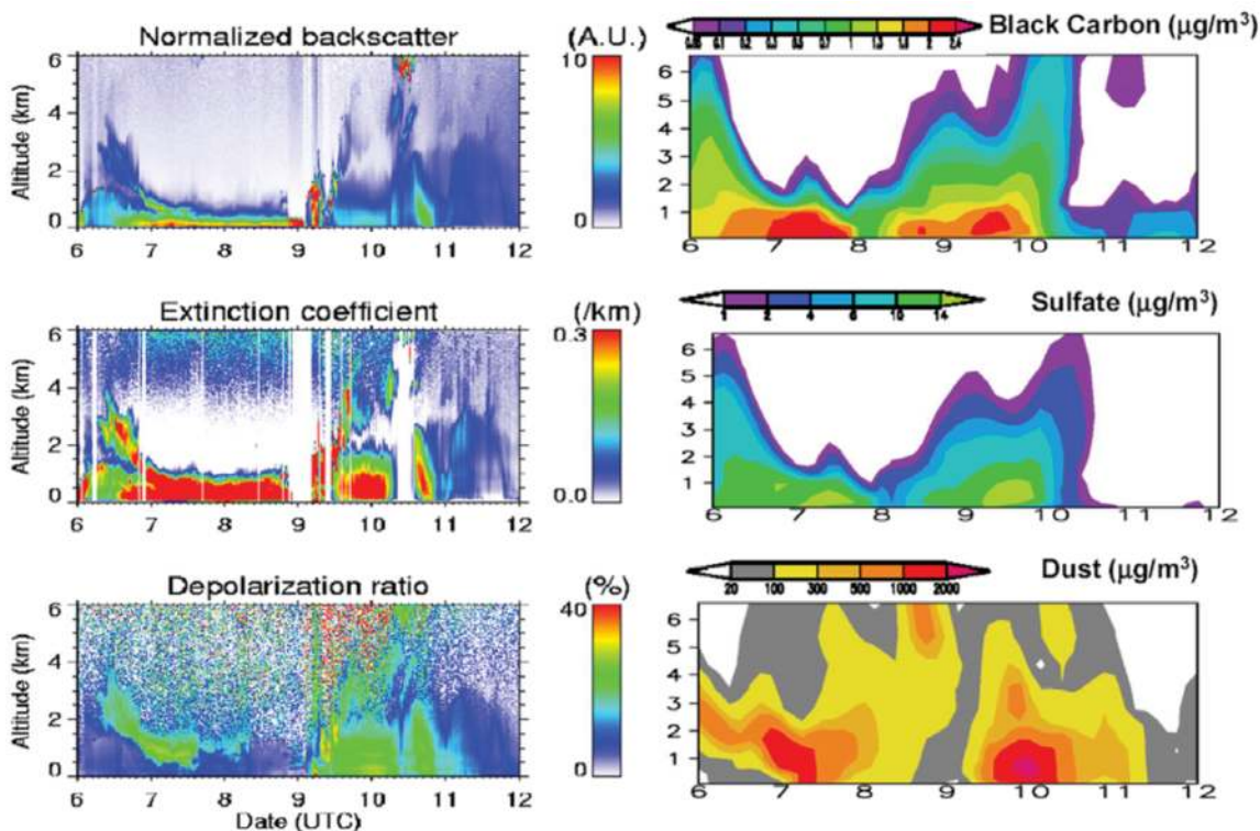
FIG. 3. (left) Lidar images over Beijing. (right) Time–height profiles of calculated mass distributions of (bottom) dust, (middle) sulfate, and (top) black carbon for Beijing using the CFORS model. Abcissa shows data (UTC) indicating day in Apr 2001.
