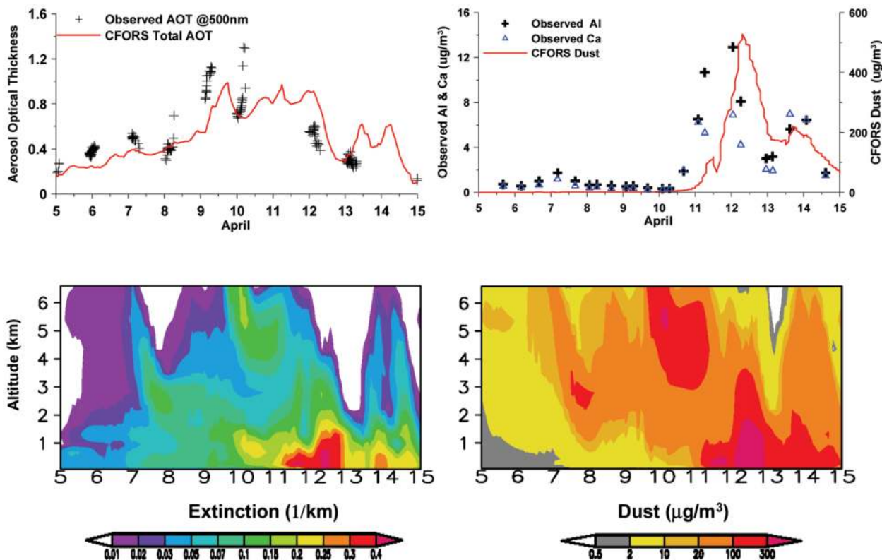
FIG. 5. (top left) Measurements of AOT on the R/V Ronald H. Brown over 5–15 Apr show values exceeding 1.0 during the height of the dust storm. (top right) Al and Ca, measured onboard, also peak at this time. In most cases model predictions follow these data closely. (bottom) Predicted vertical distributions of (left) aerosol extinction and (right) dust concentrations are shown corresponding to the Ronald H. Brown cruise track.
