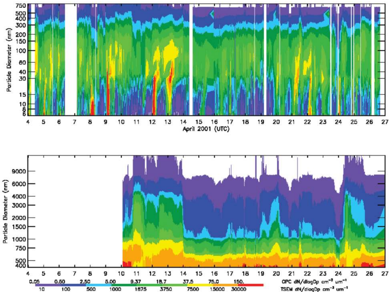
FIG. 6. (top) Electrical mobility and (bottom) optical particle (OPC) number size distributions measured at Gosan. Data are shown as timelines with particle size on the ordinate, time on the abscissa, and color contours representing the number concentration at a given size. Three distinct dust events on 10–13, 19, and 24–25 Apr are evident in the coarse mode OPC data, with simultaneous decreases in submicrometer number concentrations, especially for particles larger than 150 nm and smaller than 30 nm. The noted behavior in the submicrometer range may be attributable to precipitation scavenging of particles in air heavily influenced by cloud processing in the frontal boundary transporting the dust.
