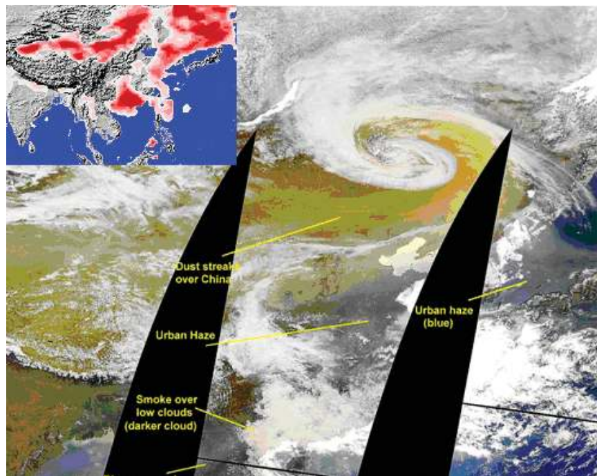
FIG. 1. The Sea-viewing Wide Field-of-View Sensor (SeaWiFS) image for 7 Apr 2001 illustrates the complexity of the aerosol distributions during large dust storms. Dust (shown in yellowish brown) is transported, along with the intense low pressure system, horizontally and vertically into the center of the low. Ahead of the front, urban pollution (brownish gray area south of the dust) is transported across Korea and Japan. During this period, widespread fires were burning in Southeast Asia, and carbonaceous aerosols associated with these fires were transported away from the continent and toward Japan in the warm sector ahead of this large cold front. Over the Pacific, these aerosols are higher than the clouds. The composite TOMS aerosol index (AI) for 7–9 Apr 2001 (upper left corner) is indicative of absorbing aerosol (either dust or black carbon). The high values of AI (indicated by dark red) over east Asia are due to dust, while those in Southeast Asia are due to biomass burning. The TOMS image shows clearly the two waves of dust associated with the storm.
