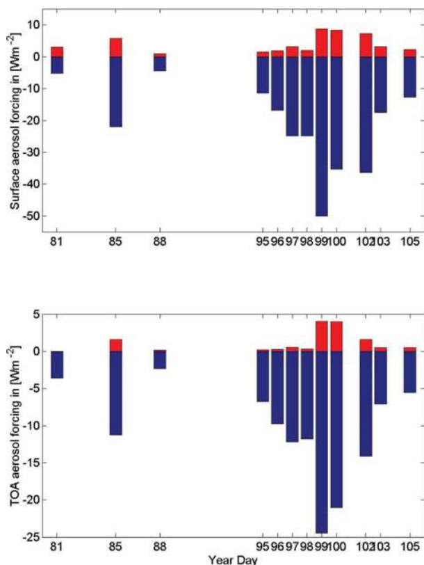
FIG. 8. Comparison between (a) the surface and (b) the TOA shortwave and IR aerosol forcing. The positive values correspond with IR forcing and negative values are for solar aerosol forcing.
