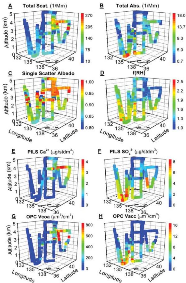
FIG. 4. Measurements aboard the NCAR C-130 on 8 Apr in the dust cloud over the Sea of Japan. This eight-panel plot is arranged into four panels of measured aerosol optical characteristics at 550 nm [(a) total aerosol light scattering, (b) total aerosol light absorption, (c) aerosol single scattering albedo, (d) f(\text{RH}) , see text] and (e)–(h) four panels of the physicochemical properties that give rise to these characteristics. Observed aerosol (e) \text{Ca}^{2+} and (f) \text{SO}_4^{2-} as a function of altitude along the flight track are based on rapid and continuous measurements with a new instrument (PILS) that captures particles ( \leq 1.5\text{-}\mu\text{m} diameter) directly into a small flow of purified water (Weber et al. 2001). Although the predominance of calcium occurred in larger particles (total calcium reached 19,000 pptv versus only 1600 pptv in particles \leq 1.5 \mu\text{m} ), the PILS data are still a reliable indication of dust because the tail of the dust distribution goes below 1.5 \mu\text{m} . (g) Coarse and (h) fine aerosol components, separated at aerodynamic particle diameter of 1 \mu\text{m} , are shown here as “dry” volumes as measured.
