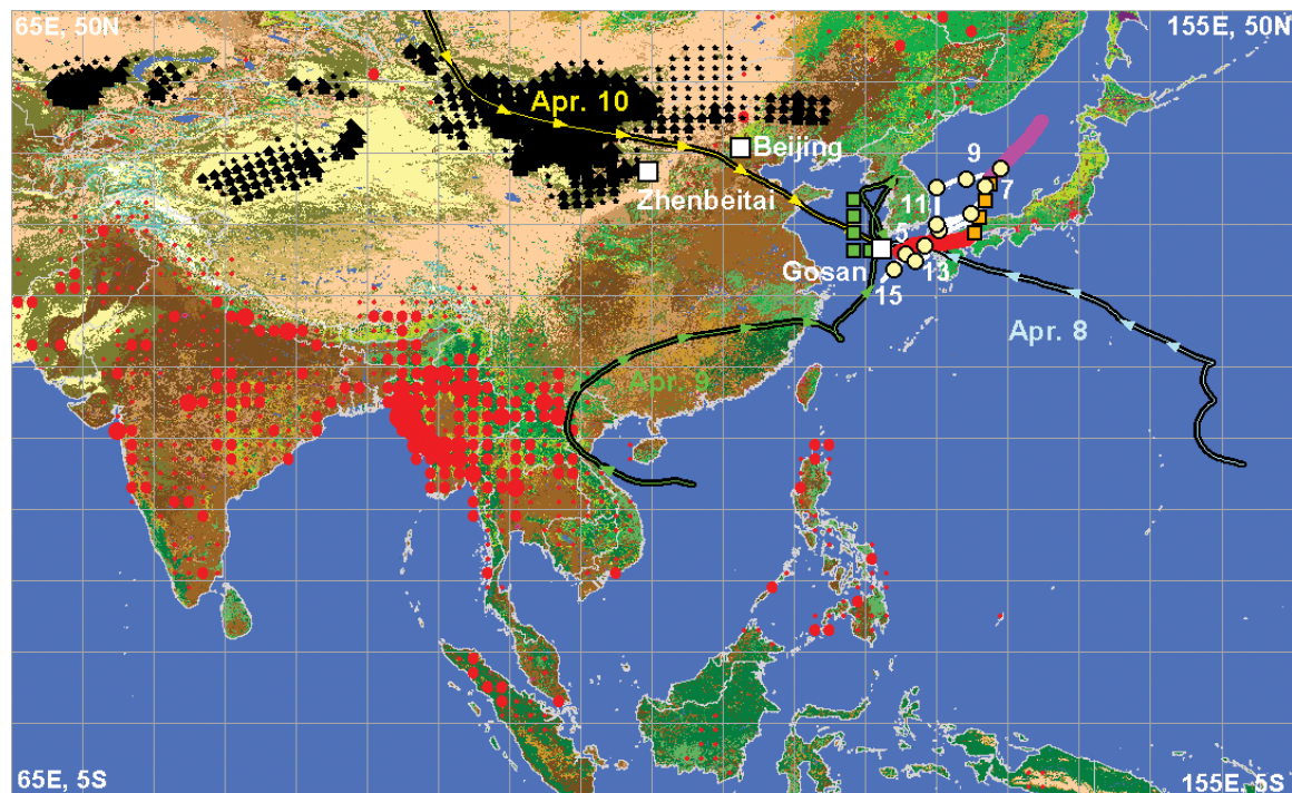
FIG. 2. Dust emissions fluxes (black) and AVHRR fire counts (red) over the period 1–20 Apr 2001. Surface measurement sites discussed in the text are shown, along with the location of the R/V Ronald H. Brown , and the flight tracks of the C-130 and Twin Otter aircraft on 8 and 12 Apr. Numbers next to the tracks indicate Apr dates. Near-surface three-dimensional trajectories were calculated by the RAMS meteorological model, as described in Uno et al. (2003). At the time that the R/V Ronald H. Brown observed the dust storm on 11 Apr it was positioned near the tip of South Korea, where trajectories were very similar to those at Gosan.
