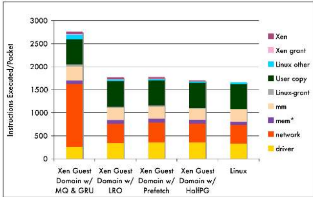
Figure 5. Guest domain cost breakdown in instructions executed/packet
