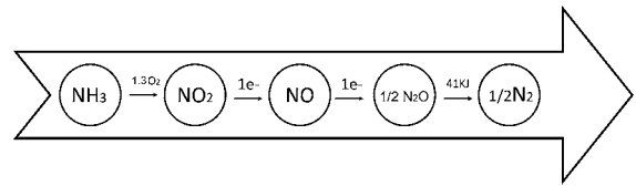
Fig. 7 CANDO process scheme (Gao et al. 2014)
