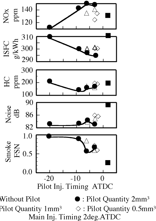
Fig. 7 Effects of close pilot injection at light load.
