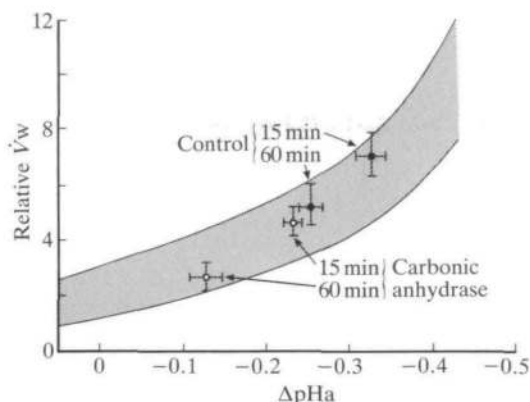
Fig. 6. The mean relationship ( \pm 1 s.e.m.) between relative ventilation ( \dot{V}_w ) and the change in arterial blood pH ( \Delta pHa ) determined from 91 measurements in 27 adult rainbow trout at various times after exhaustive exercise stress (6 min chasing) at 15°C. \dot{V}_w and \Delta pHa are expressed relative to pre-exercise resting levels. Superimposed on this relationship are shown the data (means \pm 1 s.e.m.) for the two different treatment groups at 15 and 60 min post-exercise. The experimental group ( N=12 ) received an intra-arterial infusion of 10 mg kg -1 bovine carbonic anhydrase to reduce post-exercise increases in P_{aCO_2} and decreases in pHa. The control group ( N=15 ) received only saline. (Unpublished data of C. M. Wood and R. S. Munger.)
