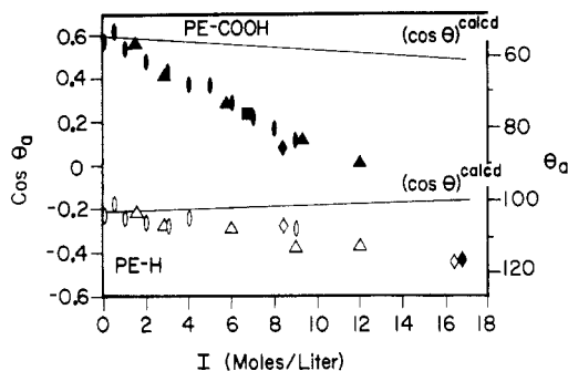
Figure 24. Effect of ionic strength ( I ) on \cos \theta_a for PE-H and PE-CO 2 H. Salts: (●, ○) NaClO 4 ; (▲, △) (NH 4 ) 2 SO 4 ; (■) NaI; (◆, ◇) AlCl 3 . The changes in \cos \theta_a predicted from changes in \gamma_{LV} alone (eq 12), using values of \gamma_{LV} for (NH 4 ) 2 SO 4 as representative, are shown for comparison.
