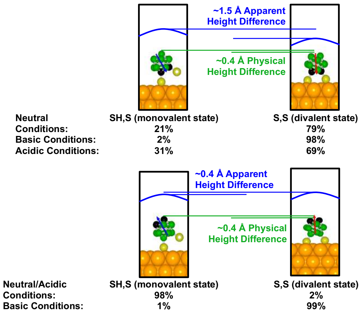
Figure 7. Binding assignments measured by scanning tunneling microscopy and scanning tunneling spectroscopy (STS). (Top) Self-assembled monolayers composed of 1,2-(HS) 2 -1,2-C 2 B 10 H 10 ( 1O2 ) form into (left) a thiol/thiolate state (monovalent form) and (right) a dithiolate state (divalent form) that differ in apparent height in scanning tunneling microscope images. (Bottom) Monolayers composed of 9,12-(HS) 2 -1,2-C 2 B 10 H 10 ( 9O12 ) form into (left) an adsorbed monothiol/monothiolate (monovalent) state, under acidic and neutral conditions and (right) a dithiolate (divalent) state that differ in measured apparent height, as shown for the conditions
