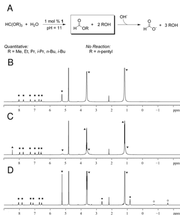
Figure 2 (A) Reaction and substrate scope for orthoformate hydrolysis in the presence of catalytic 1 . (B-D) All spectra taken with 50 equiv. of triethyl orthoformate with respect to 1 at pD 11.0, 100 mM \text{K}_2\text{CO}_3 , 22 °C, in \text{D}_2\text{O} . (B) Initial spectrum. (C) Spectrum after 60 minutes. (D) Spectrum of 1 with 2 equiv. \text{NEt}_4^+ after 60 minutes. Key: 1 (■), \text{HC(OEt)}_3 (▼), \text{NEt}_4^+ (● exterior, ○ interior), product \text{HCO}_2\text{H} (▲).
