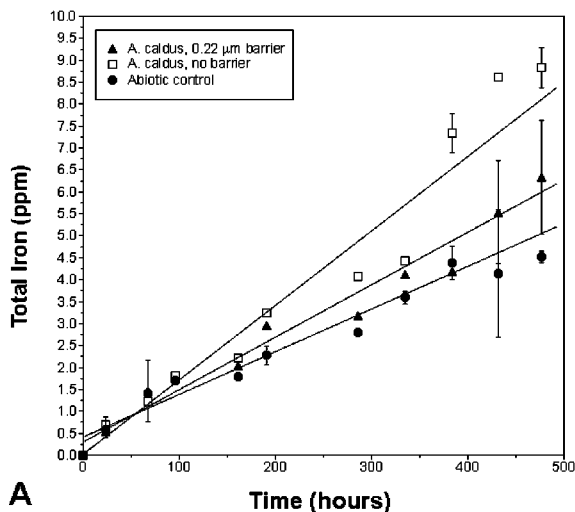
FIG. 4. Results of FeAsS oxidation experiments in which Acidithiobacillus caldus was added to reaction vessels and allowed either direct contact with the mineral, or was separated from the mineral with a 0.2 μm filter.
