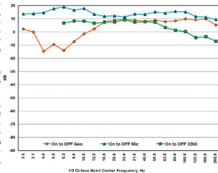
Figure 28. 1/3 octave difference
