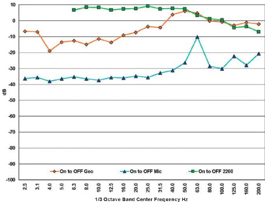
Figure 26. 1/3 octave difference
