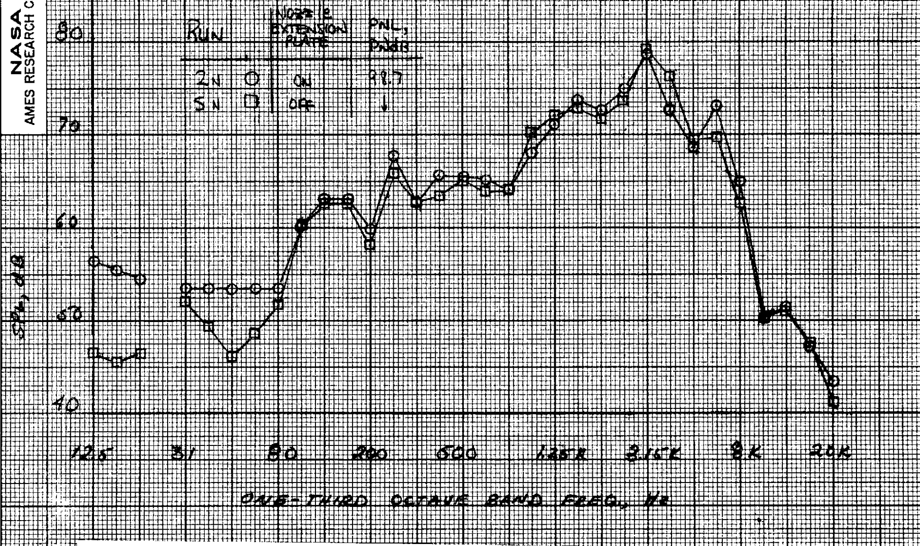
(b) Sideline frequency spectra; S/L angle = 50°; V J = 216 m/s (710 fps).
