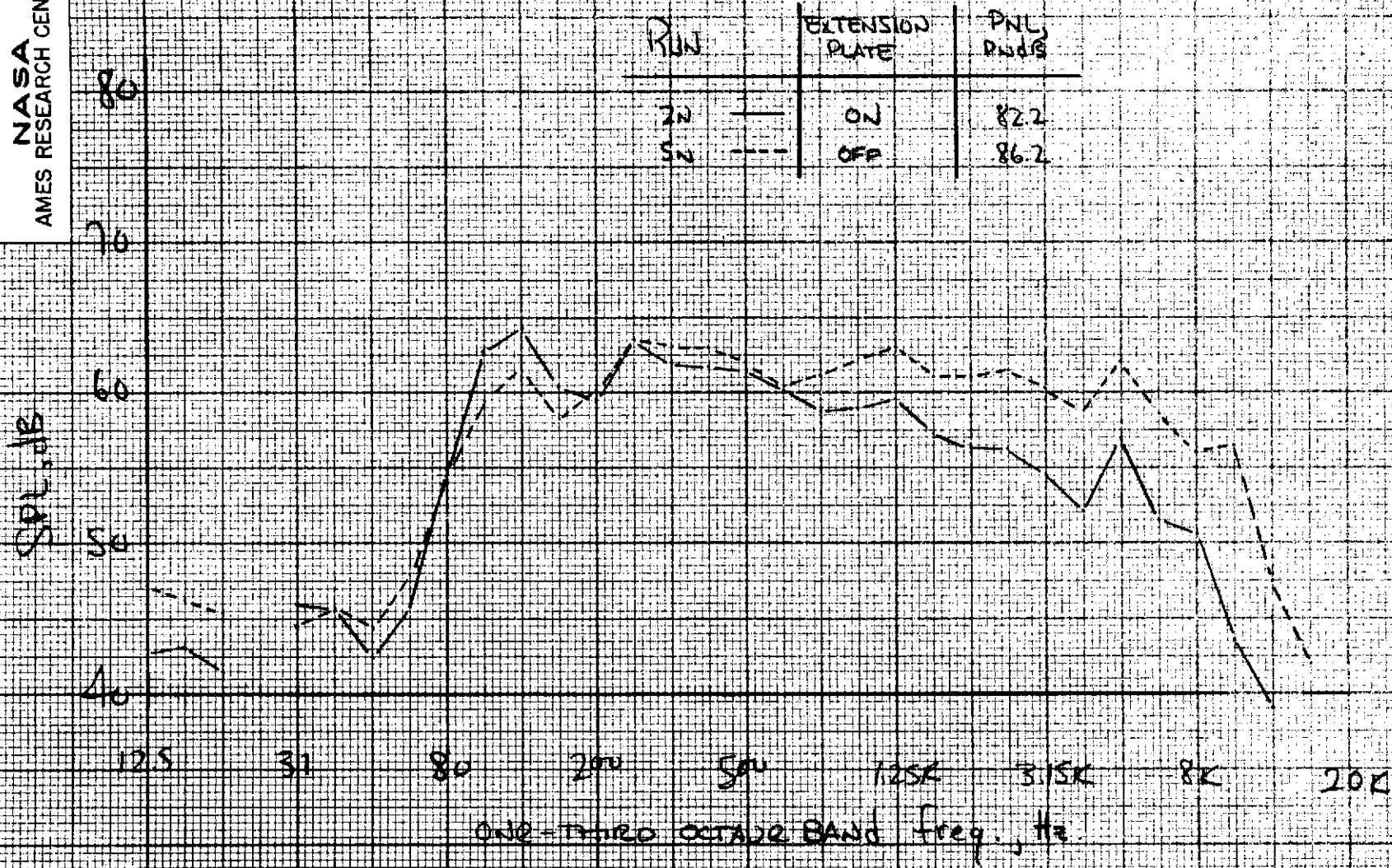
(c) Frequency spectra, U/W angle = 110^\circ , V_j = 157 m/s (513 fps).
