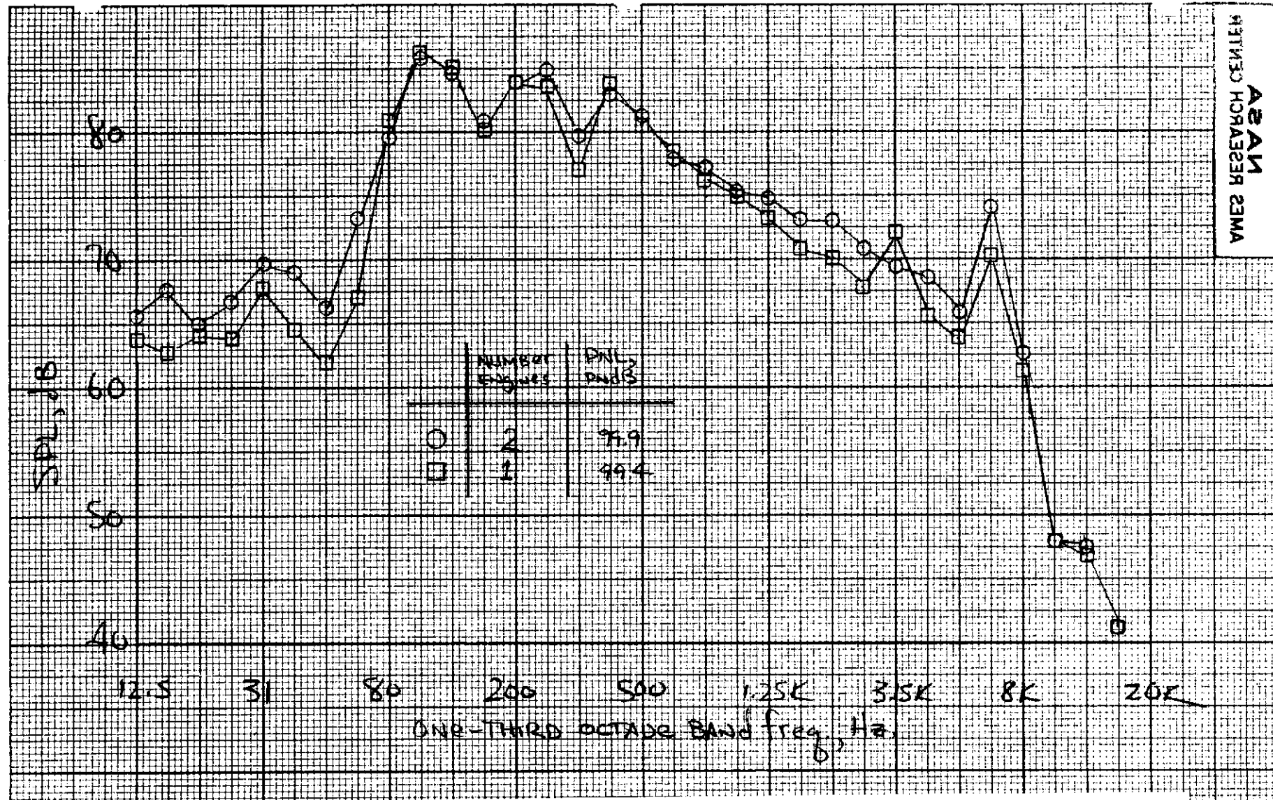
(c) Frequency spectra, U/W angle = 110^\circ , V_T = 247 m/s (810 fps).
