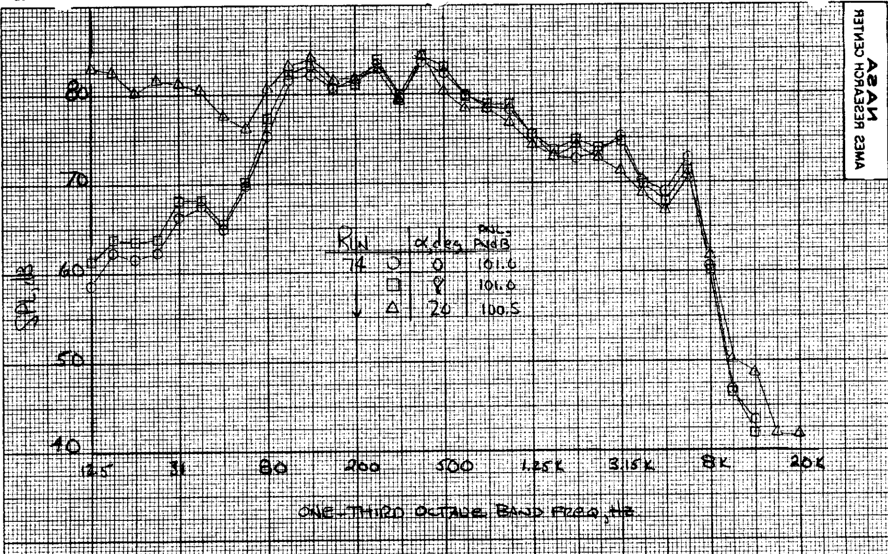
Figure 15.— Variation of underwing frequency spectra with angle of attack. Nozzle "D"; \delta_f = 75^\circ ; V_j = 254 m/s (835 fps); V_\infty = 17.2 m/s (56.5 fps); \eta_{CO} = 11.43 percent; U/W angle = 110^\circ .
